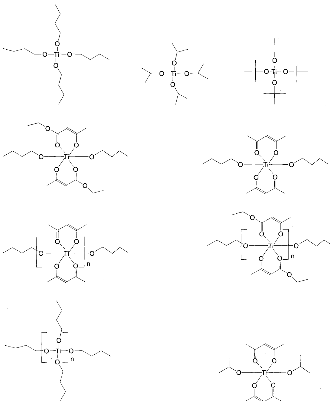
Figure 3: Examples of Titanate Compound
