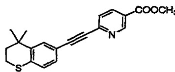
Tazoretene
