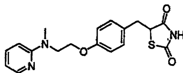
Rosiglitazone
