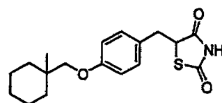
Ciglitazone
