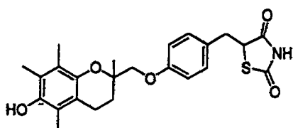
Troglitazone
