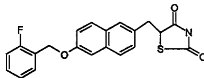
MCC-555
