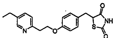
Pioglitazone
