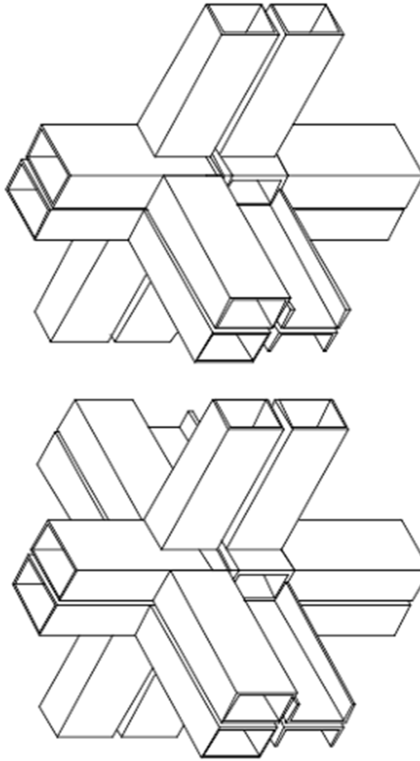
ISOMETRIC VIEW OF TYPE 1 COLUMN SPLICE JOINT ISOMETRIC VIEW OF TYPE 2 COLUMN SPLICE JOINT
