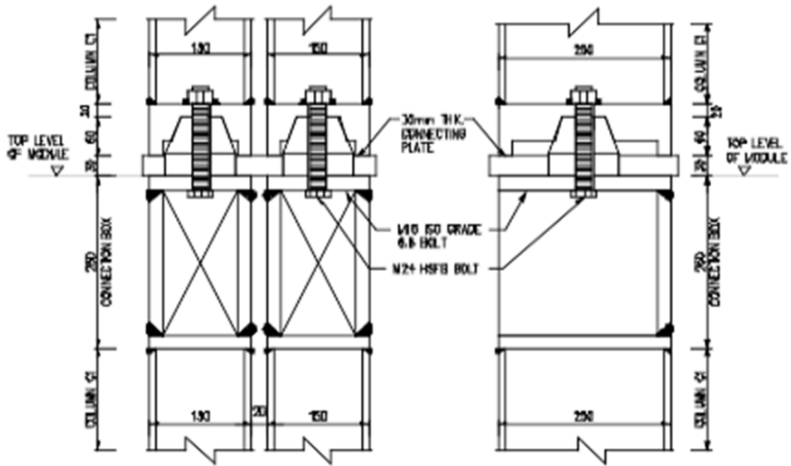
TYPE 1 COLUMN SPLICE
