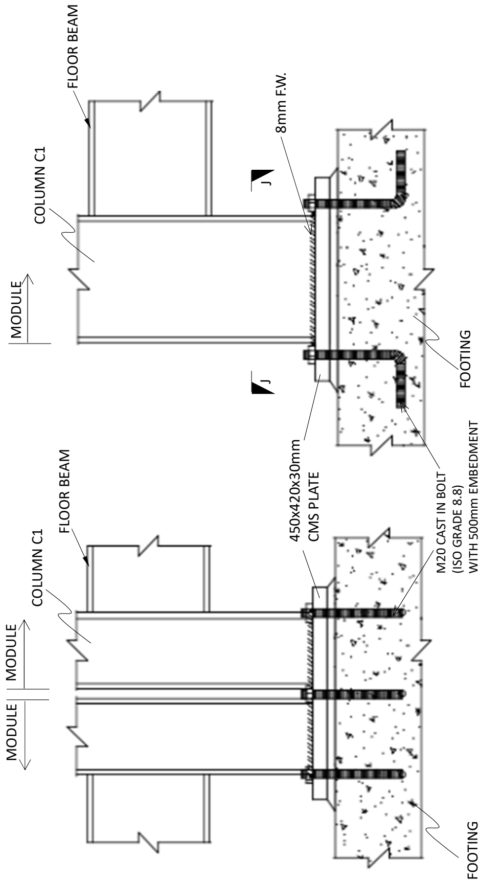
BASE FIXING FOR INTERIOR COLUMN TO FOOTINGS
