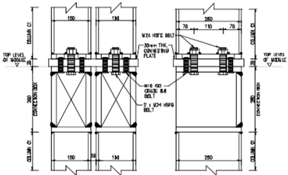
TYPE 2 COLUMN SPLICE
