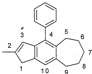
2-Methyl-4-phenyl-1,5,6,7,8, 9-hexahydro-cyclohepta[f]in dene
