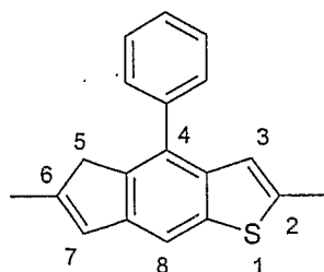
2,6-Dimethyl-4-phenyl-5 H -1-thia-s-indacene
