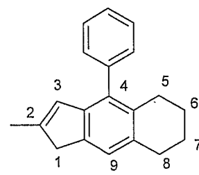
2-Methyl-4-phenyl-5,6,7,8-tetrahydro-1 H -cyclopenta[ b ]naphthalene
