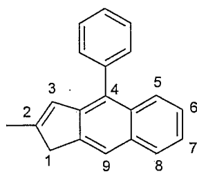
2-Methyl-4-phenyl-1 H -cyclopenta[ b ]naphthalene
