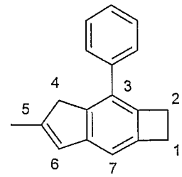
5-Methyl-3-phenyl-2,4-dihydro-1 H -cyclobuta[ f ]indene
