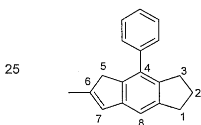
6-Methyl-4-phenyl-1,2,3,5-tetrahydro-s-indacene
