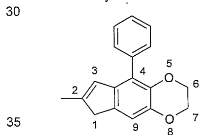
2-Methyl-4-phenyl-6,7-dihydro-1 H -5,8-dioxacyclopenta[ b ]naphthalene
