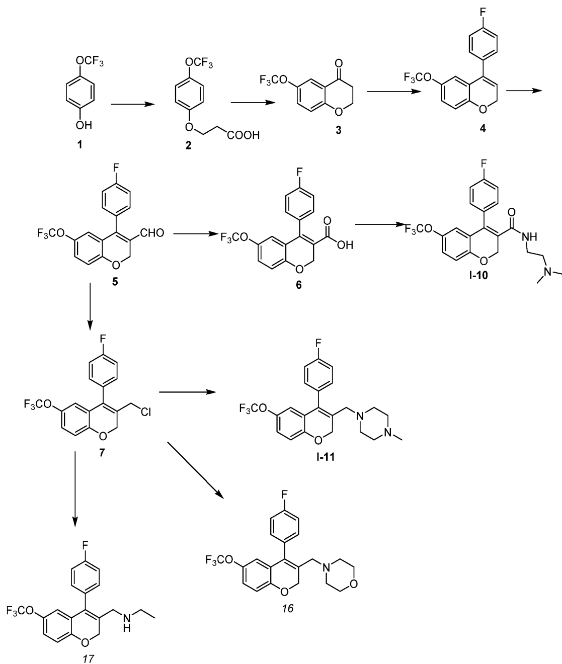
Example 1: N-(2-(dimethylamino)ethyl)-4-(4-fluorophenyl)-6-(trifluoromethoxy)-2H-chromene-3-carboxamide
