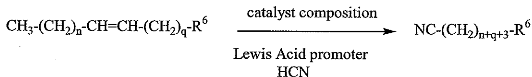
Formula V
