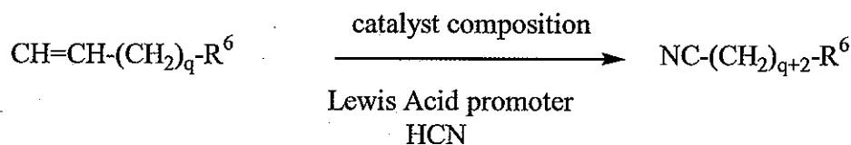
Formula VII
