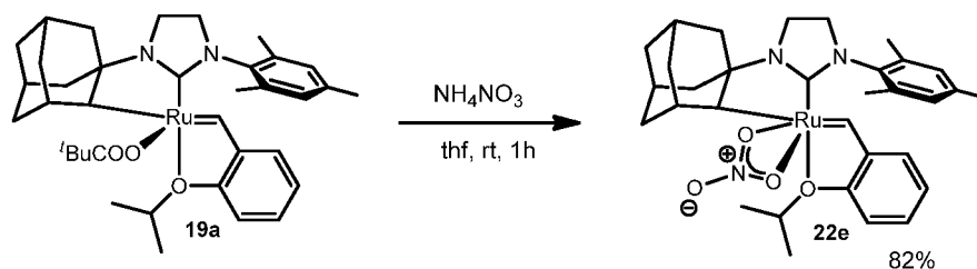
Scheme 18
