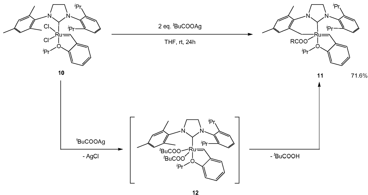
Scheme 6
