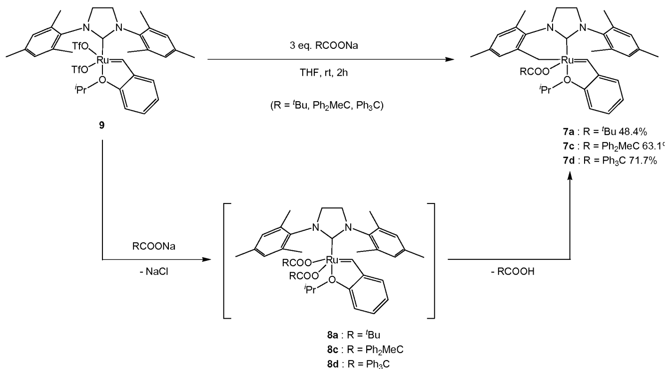
Scheme 5
