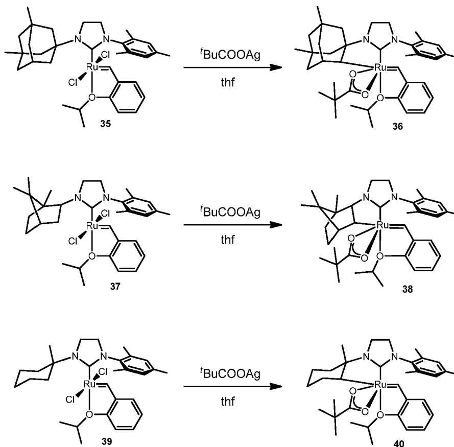
Scheme 20
