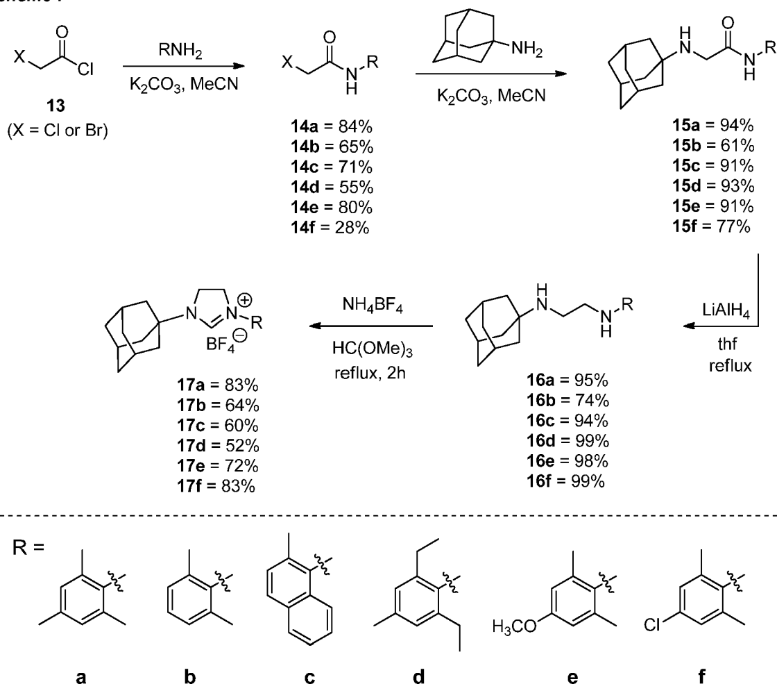
Scheme 7
