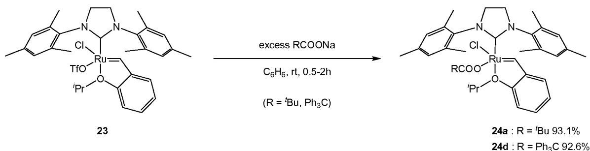
Scheme 13
