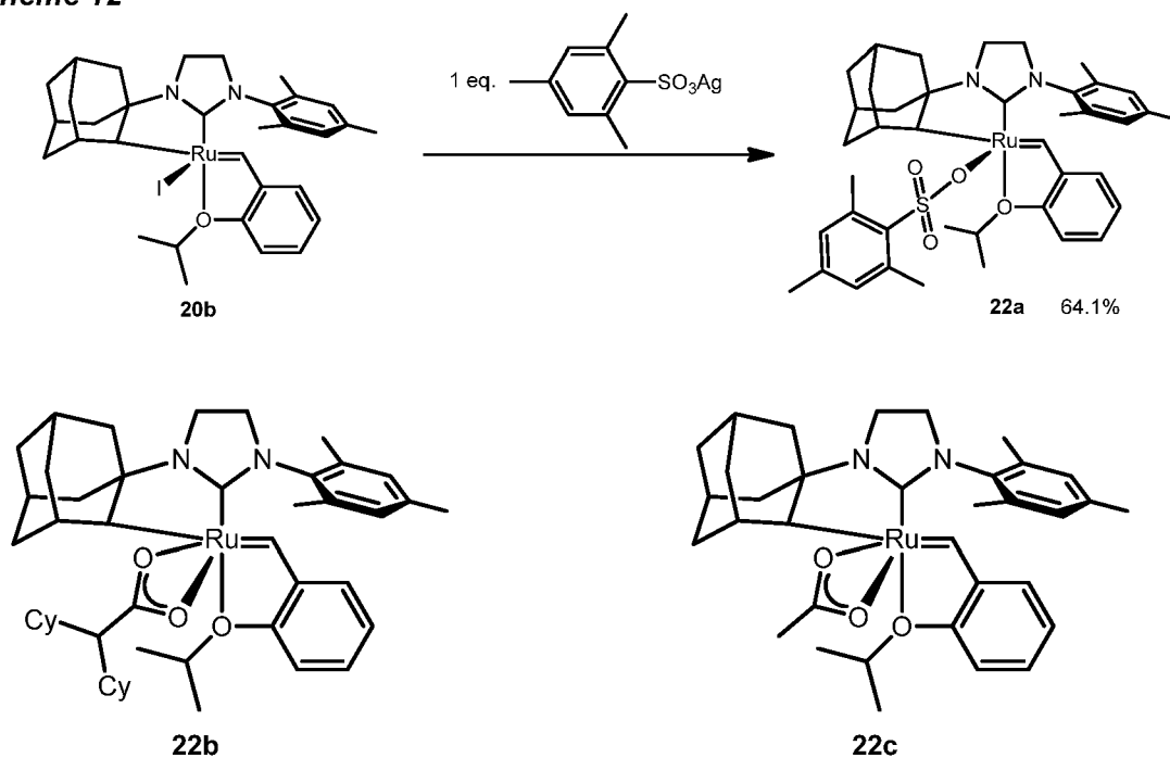
Scheme 12
