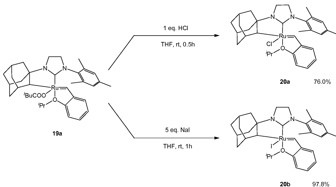
Scheme 10
