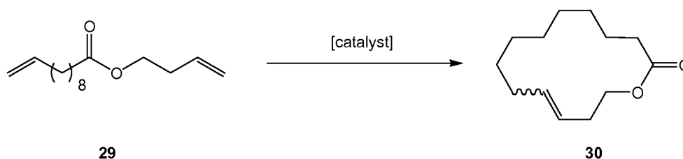
Scheme 16
