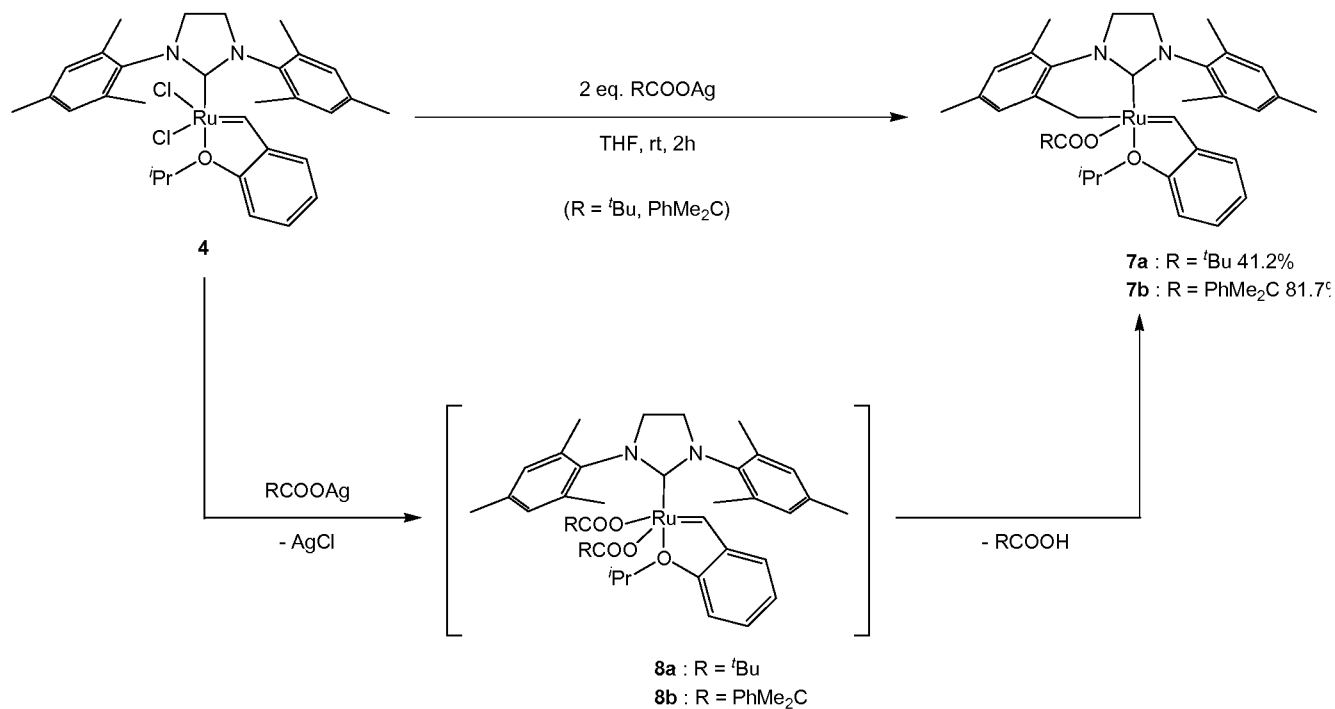
Scheme 4
