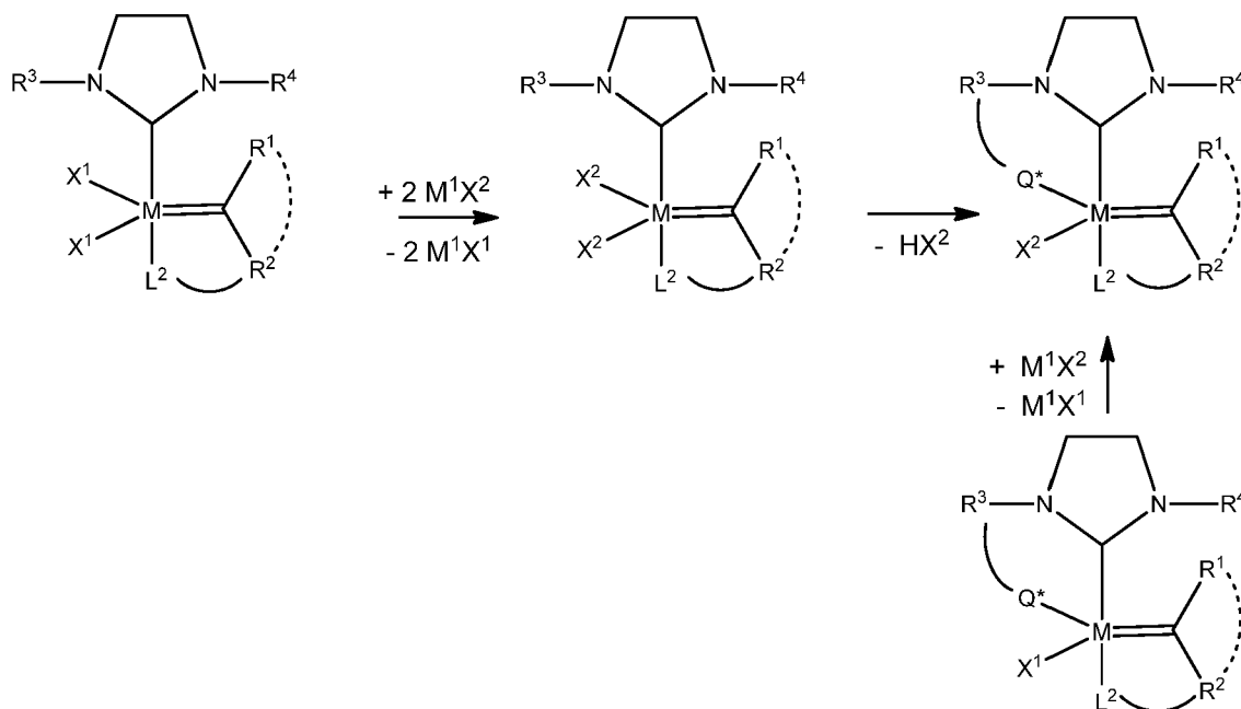
Scheme 3. Synthetic Procedure
