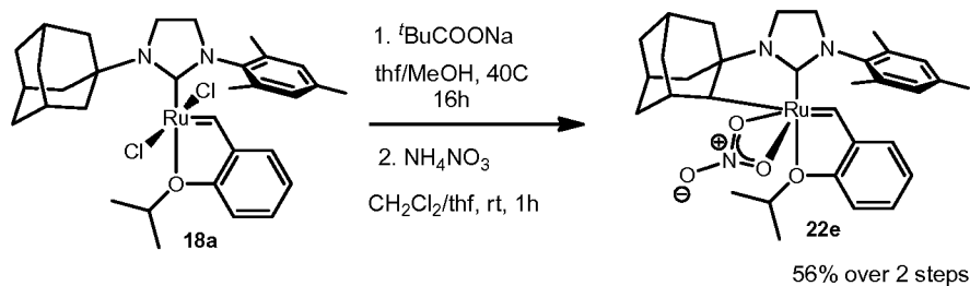
Scheme 18
