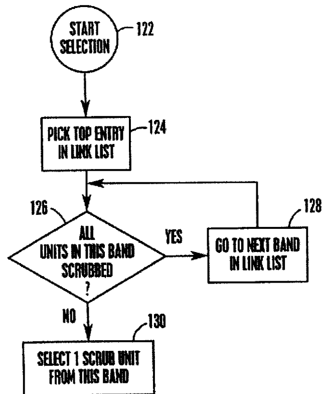
Fig. 10 Divide The Disk Into Bands - Selection Algorithm
