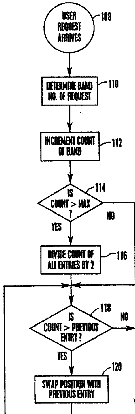
Fig. 9 Divide The Disk Into Bands - Table Maintenance
