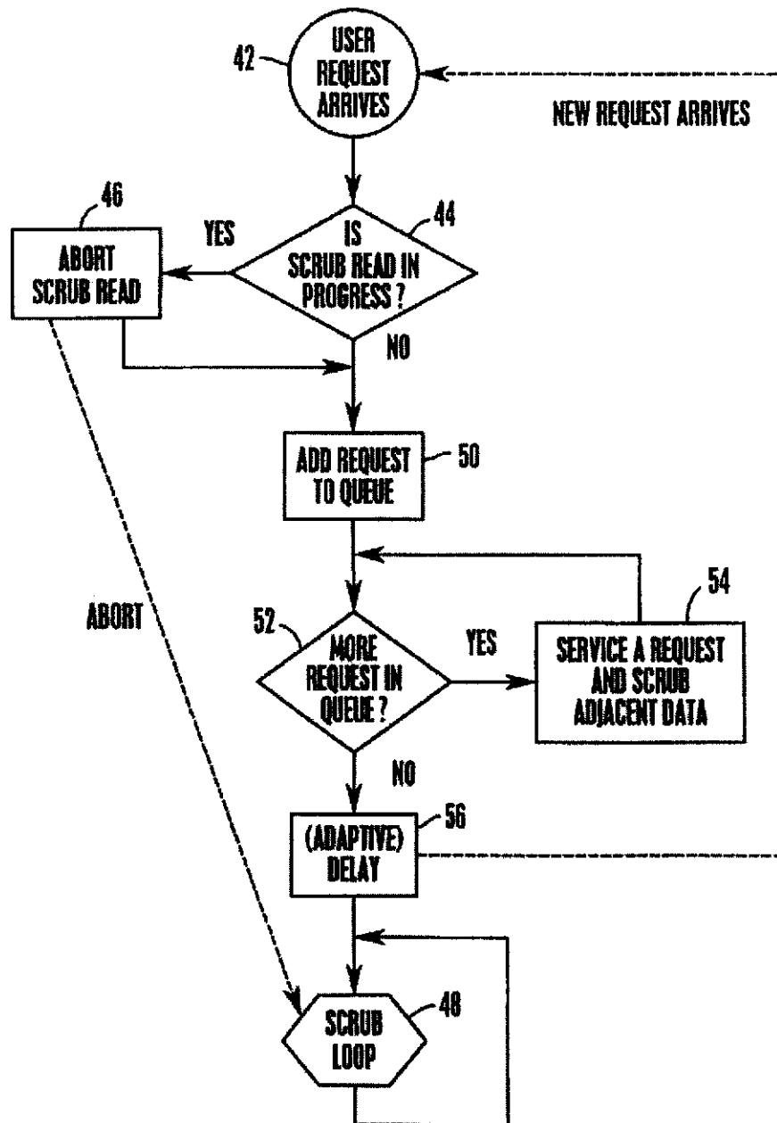
Fig. 4 Interrupt of Scrub with Delay, opportunistic options
