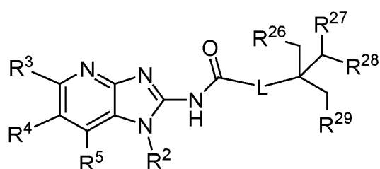
Formula A-20
