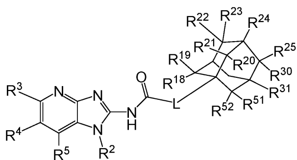
Formula A-40
