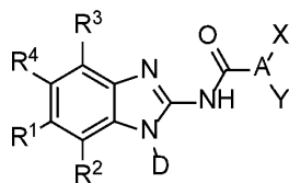
Formula B-7
