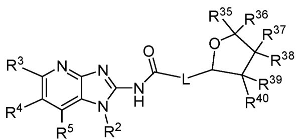
Formula A-34
