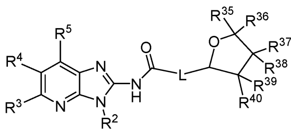
Formula A-35
