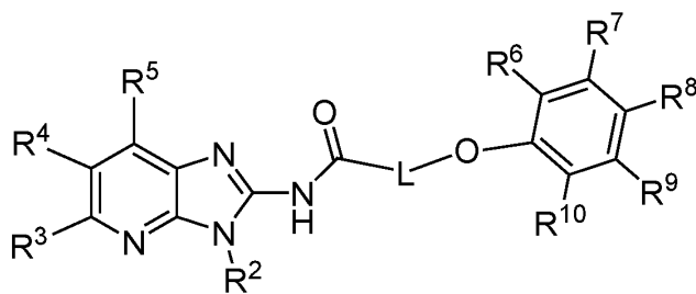
Formula A-8
