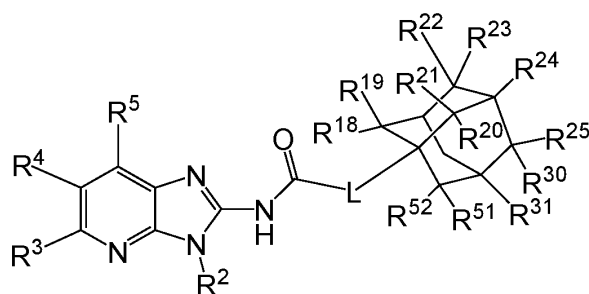
Formula A-41
