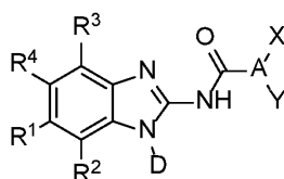
Formula 9
