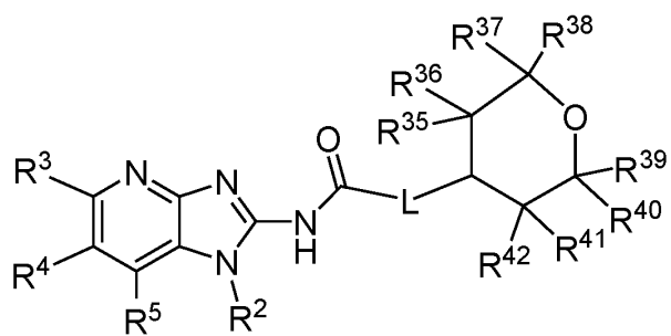
Formula A-30
