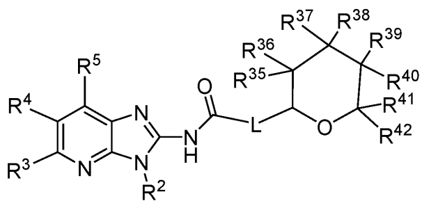
Formula A-29
