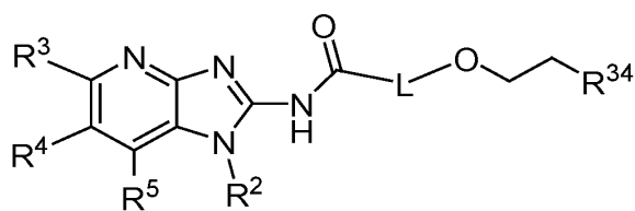
Formula A-26
