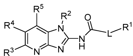
Formula A-5
