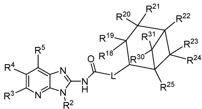
Formula A-19
