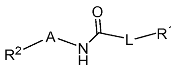
Formula A-2
