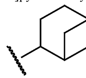
bicyclo[3.1.1]heptan-2-yl
