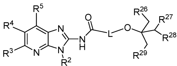
Formula A-23
