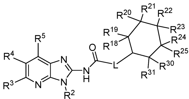
Formula A-15
