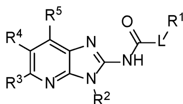
Formula A-42
