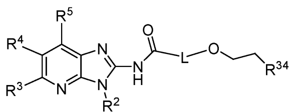
Formula A-27
