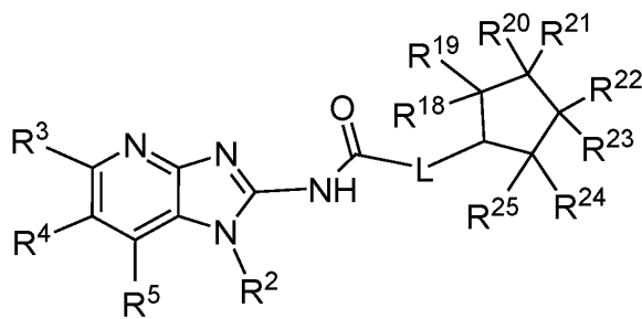
Formula A-11
