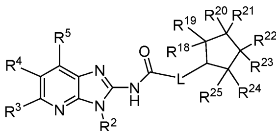
Formula A-10
