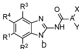
Formula 8b
