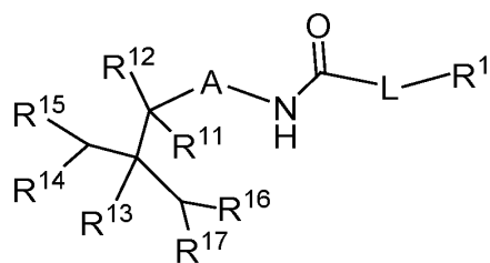
Formula A-4
