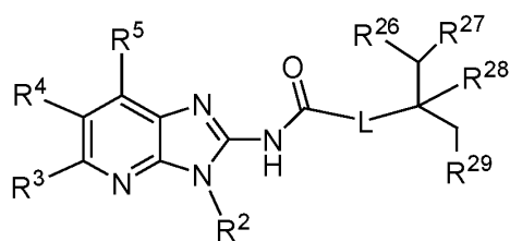
Formula A-25
