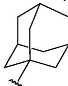
adamantan-1-yl
