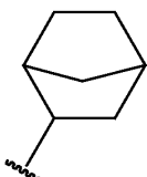
bicyclo[2.2.1]heptan-2-yl
