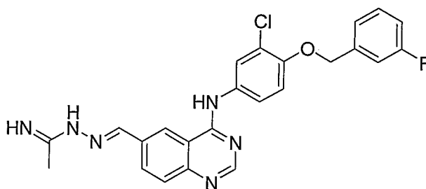
(E)-N-((4-(4-(3-Fluorobenzoyloxy)-3-chlorophenylamino)-quinazolin-6-yl)-methyleneamino)-acetamide
