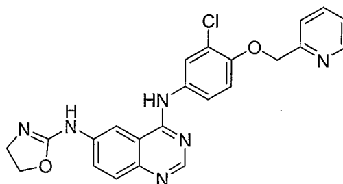
N4-[3-Chloro-4-(pyridin-2-ylmethoxy)-phenyl]-N6-(4,5-dihydrooxazol-2-yl)-quinazoline-4,6-diamine
