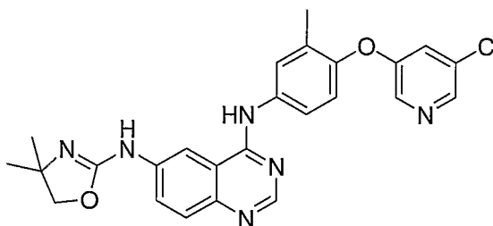
N4-[4-(5-Chloropyridin-3-yloxy)-3-methyl-phenyl]-N6-(4,4-dimethyl-4,5-dihydro-oxazol-2-yl)-quinazoline-4,6-diamine
