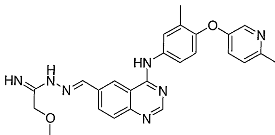
(E)-N-(4-(3-Methyl-4-(6-methylpyridin-3-yloxy)phenylamino)quinazolin-6-yl)methyleneamino-2-methoxyacetamide
