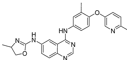
N6-(4-Methyl-4,5-dihydrooxazol-2-yl)-N4-[3-methyl-4-(6-methylpyridin-3-yloxy)-phenyl]-quinazoline-4,6-diamine
