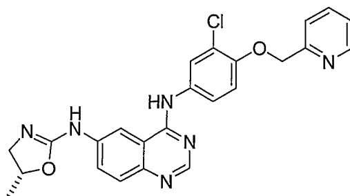
(R)-N4-[3-Chloro-4-(pyridin-2-ylmethoxy)-phenyl]-N6-(5-methyl-4,5-dihydro-oxazol-2-yl)-quinazoline-4,6-diamine
