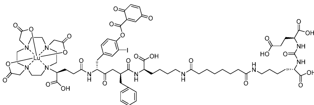
Adduct Compound Structure A1
