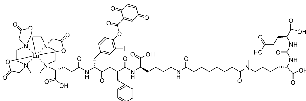
Adduct Compound Structure A2
