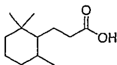
3-(2,2,6-trimethylcyclohexyl)propanoic acid
