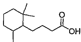
4-(2,2,6-trimethylcyclohexyl)butanoic acid
