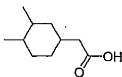
2-(3,4-dimethylcyclohexyl)acetic acid
