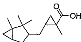
1-methyl-2-((1,2,2-trimethylbicyclo[3.1.0]hexan-3-yl)methyl)cyclopropanecarboxylic acid.
