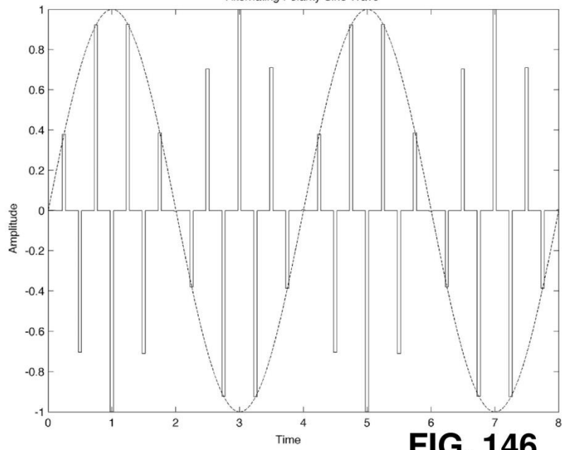
Alternating Polarity Sine Wave
