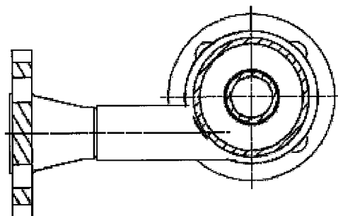
Fig. 5 Section C-C
