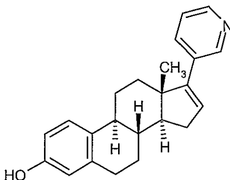
17-(3-Pyridyl)oestra-1,3,5(10),16-tetraen-3-ol
