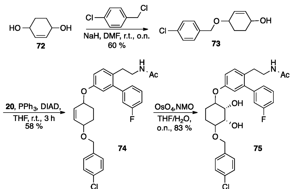
Scheme 7: Synthesis of 75.
