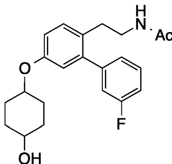
N -(2-(3'-fluoro-5-((4-hydroxycyclohexyl)oxy)-[1,1'-biphenyl]-2-yl)ethyl)acetamide ( 48 )
