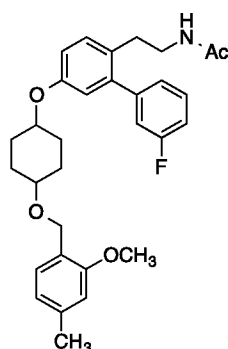
N -(2-(3'-fluoro-5-((4-((2-methoxy-4-methylbenzyl)oxy)cyclohexyl)oxy)-[1,1'-biphenyl]-2-yl)ethyl)acetamide (68)
