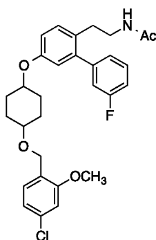
N -(2-(5-((4-((4-chloro-2-methoxybenzyl)oxy)cyclohexyl)oxy)-3'-fluoro-[1,1'-biphenyl]-2-yl)ethyl)acetamide (65)
