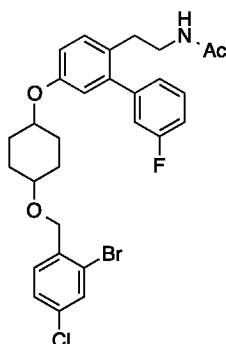
N -(2-(5-((2-bromo-4-chlorobenzyl)oxy)cyclohexyl)oxy)-3'-fluoro-[1,1'-biphenyl]-2-yl)ethyl)acetamide (66)
