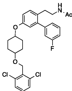
N -(2-(5-((4-((2,6-dichlorobenzyl)oxy)cyclohexyl)oxy)-3'-fluoro-[1,1'-biphenyl]-2-yl)ethyl)acetamide (64)
