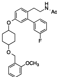
N -(2-(3'-fluoro-5-((4-((2-methoxybenzyl)oxy)cyclohexyl)oxy)-[1,1'-biphenyl]-2-yl)ethyl)acetamide (52)
