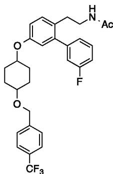
N -(2-(3'-fluoro-5-((4-((4-(trifluoromethyl)benzyl)oxy)cyclohexyl)oxy)-[1,1'-biphenyl]-2-yl)ethyl)acetamide (62)
