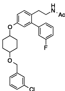
N -(2-(5-((4-((3-chlorobenzyl)oxy)cyclohexyl)oxy)-3'-fluoro-[1,1'-biphenyl]-2-yl)ethyl)acetamide (55)
