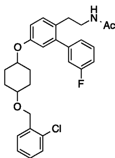
N -(2-(5-((4-((2-chlorobenzyl)oxy)cyclohexyl)oxy)-3'-fluoro-[1,1'-biphenyl]-2-yl)ethyl)acetamide (51)
