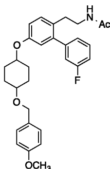
N -(2-(3'-fluoro-5-((4-((4-methoxybenzyl)oxy)cyclohexyl)oxy)-[1,1'-biphenyl]-2-yl)ethyl)acetamide (60)
