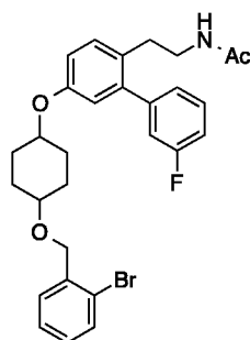
N -(2-(5-((4-((2-bromobenzyl)oxy)cyclohexyl)oxy)-3'-fluoro-[1,1'-biphenyl]-2-yl)ethyl)acetamide ( 50 )
