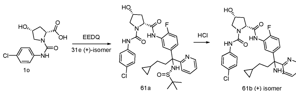
Scheme 61
