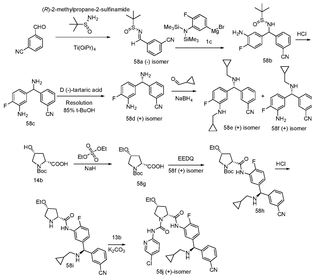
Scheme 58
