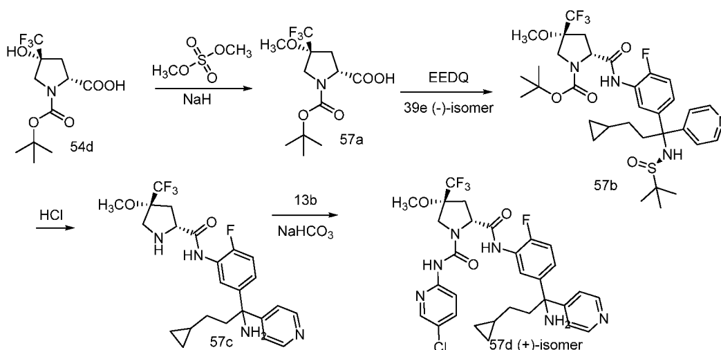
Scheme 57
