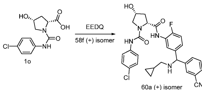
Scheme 60
