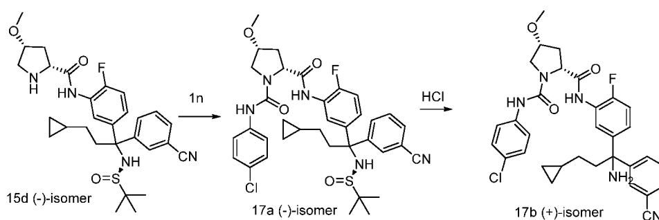
Scheme 17
