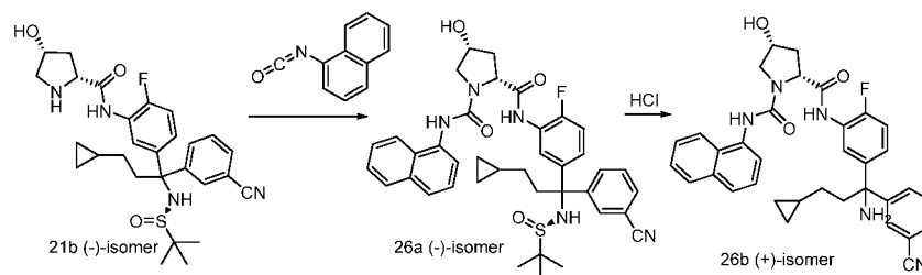
Scheme 26
