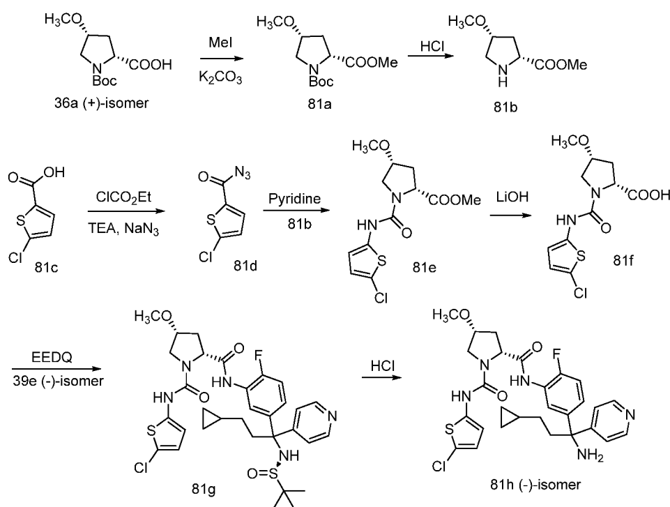
Scheme 81
