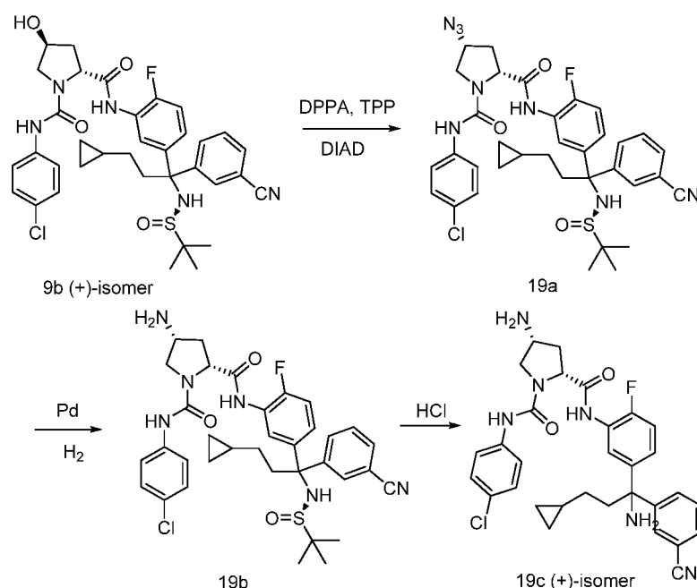
Scheme 19
