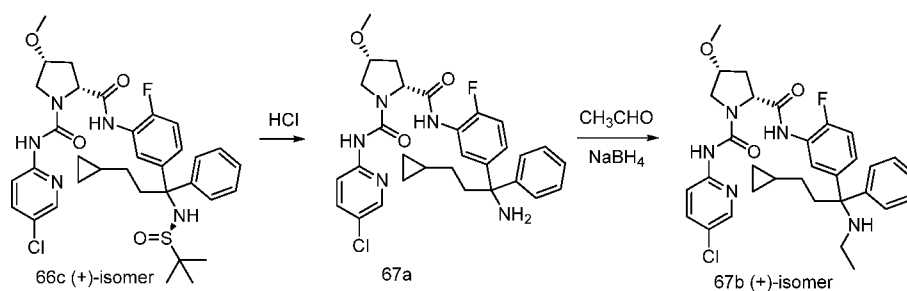
Scheme 67
