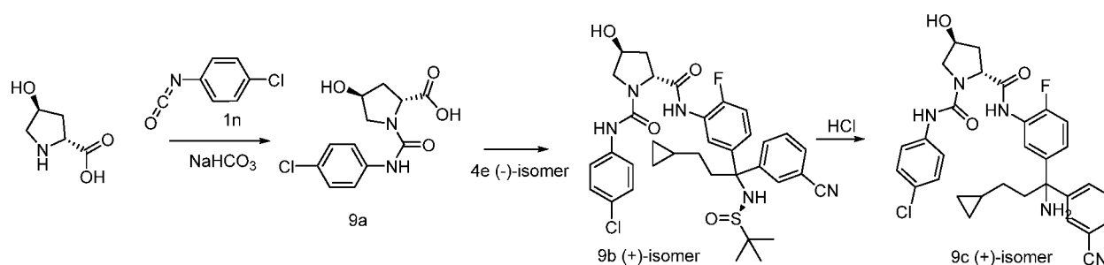
Scheme 9
