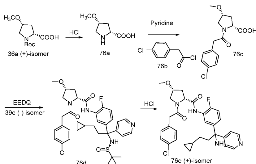
Scheme 76
