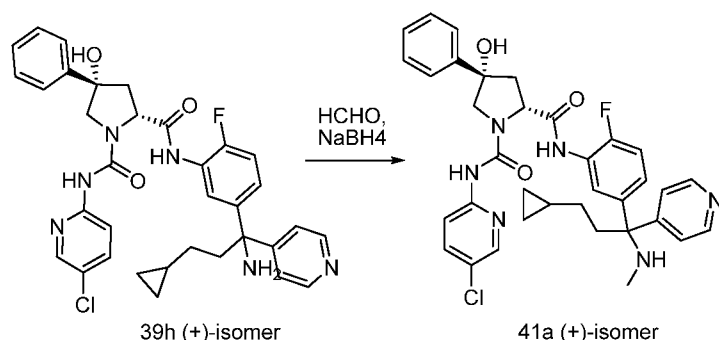
Scheme 41
