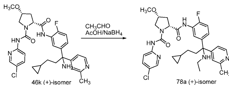
Scheme 78
