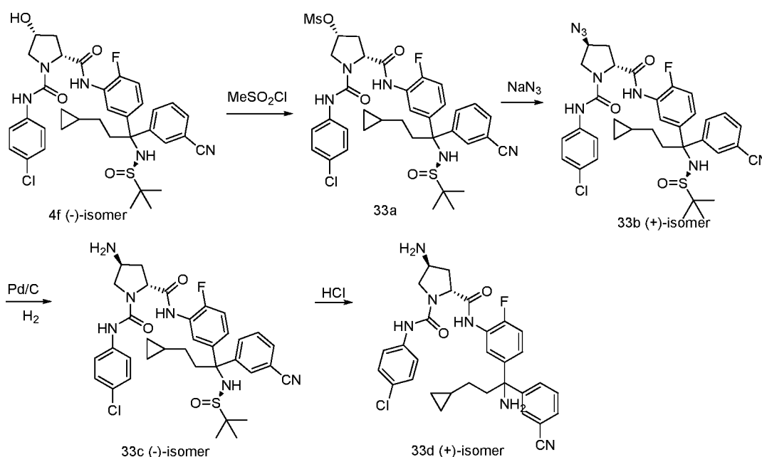
Scheme 33
