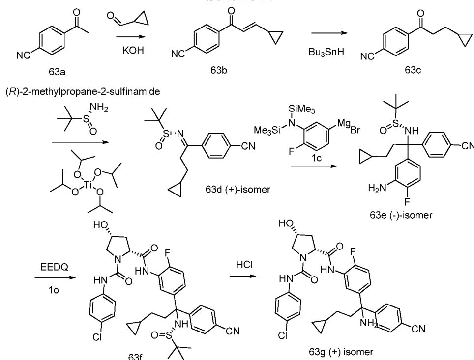
Scheme 63
