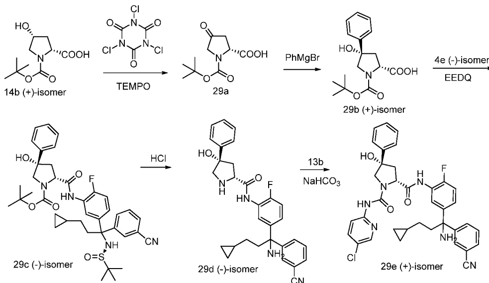
Scheme 29
