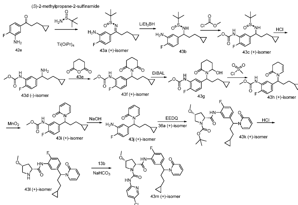
Scheme 43
