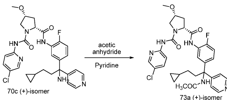
Scheme 73
