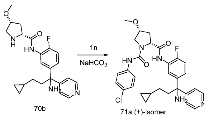
Scheme 71
