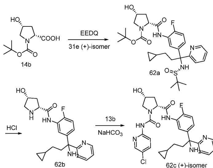
Scheme 62
