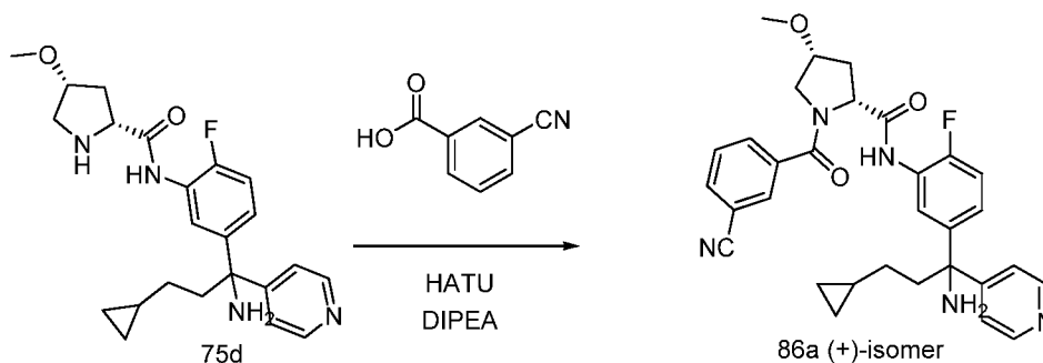
Scheme 86
