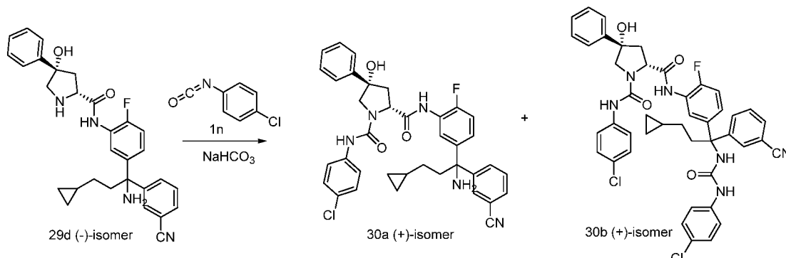
Scheme 30
