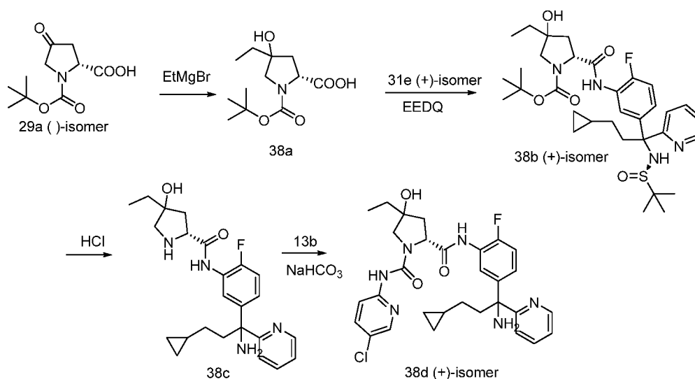
Scheme 38
