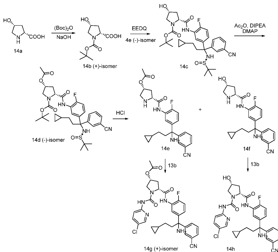
Scheme 14
