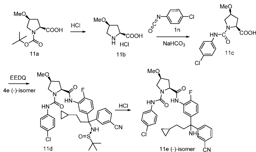
Scheme 11
