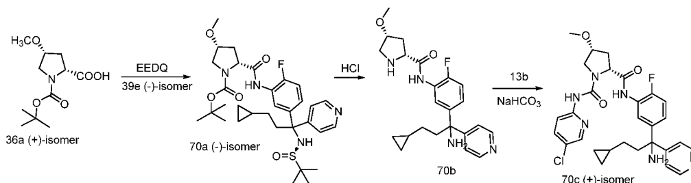
Scheme 70
