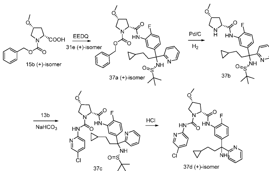
Scheme 37
