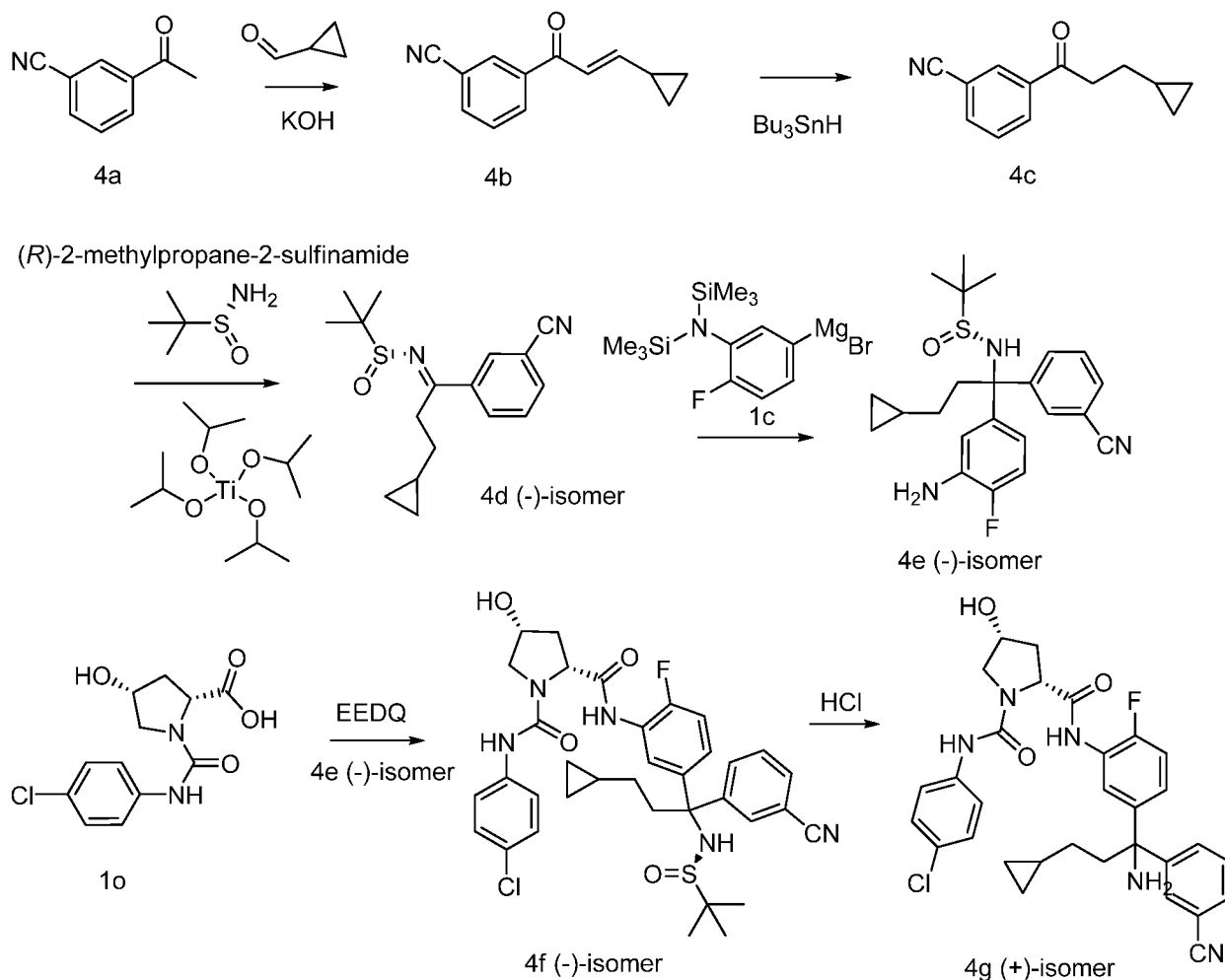
Scheme 4
