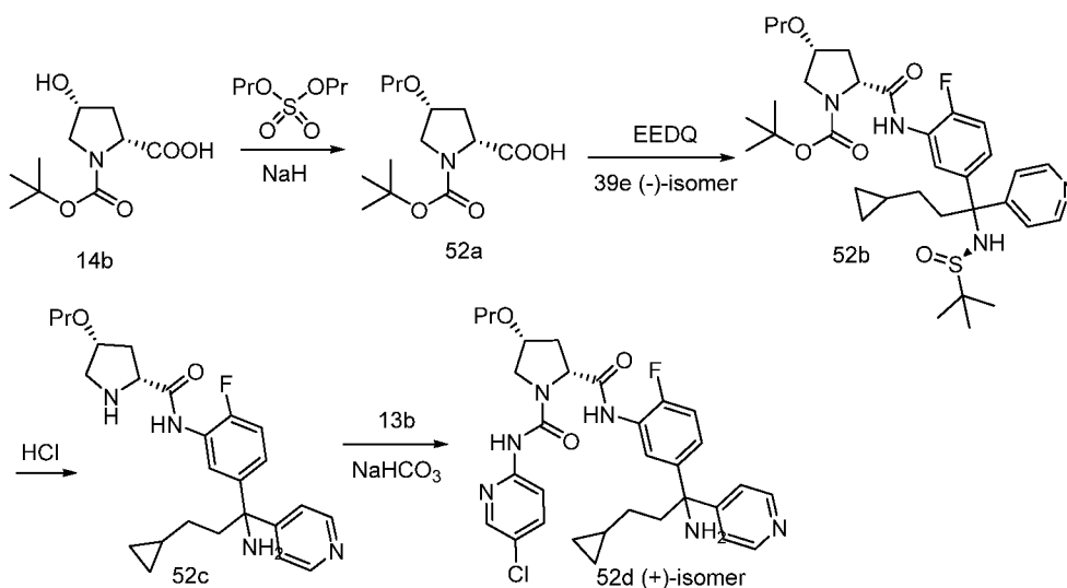
Scheme 52
