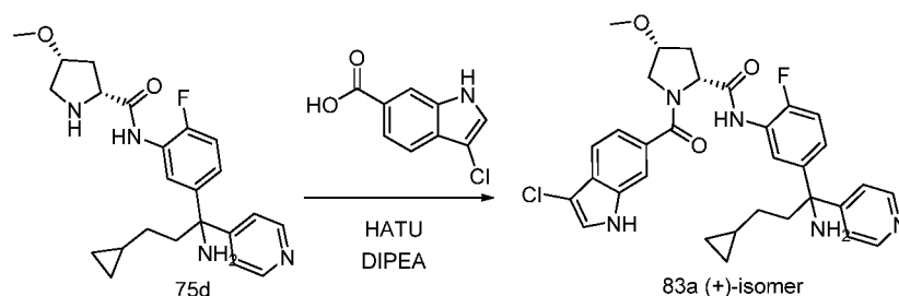
Scheme 83
