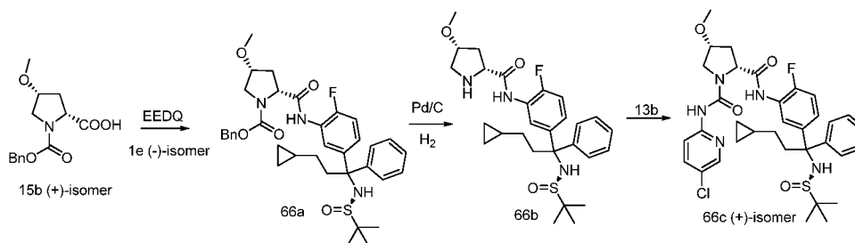
Scheme 66
