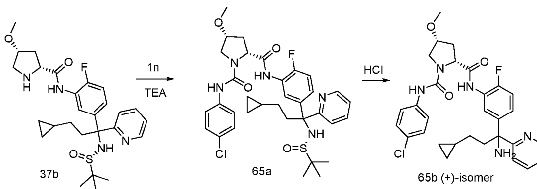
Scheme 65
