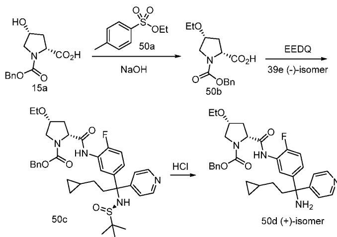
Scheme 50
