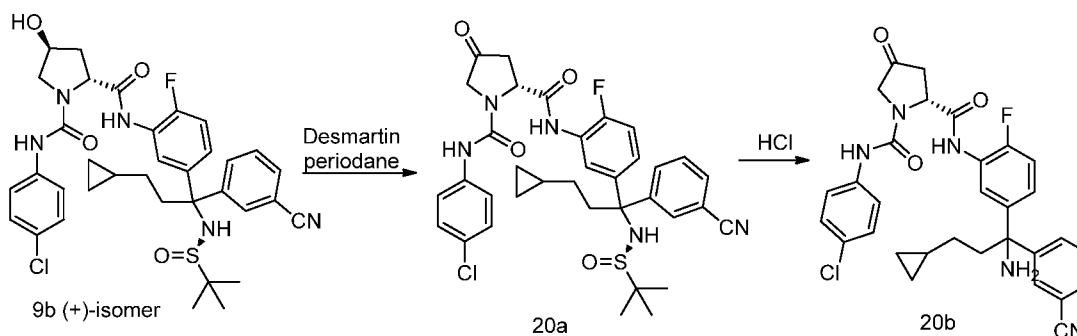
Scheme 20
