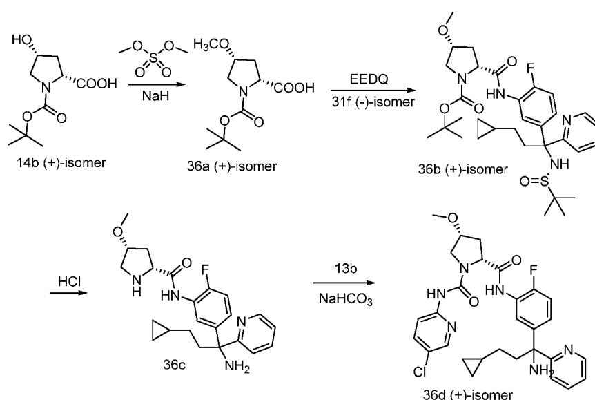
Scheme 36
