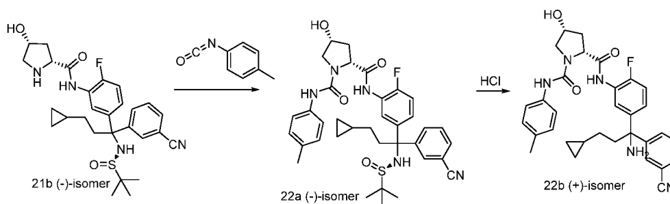
Scheme 22
