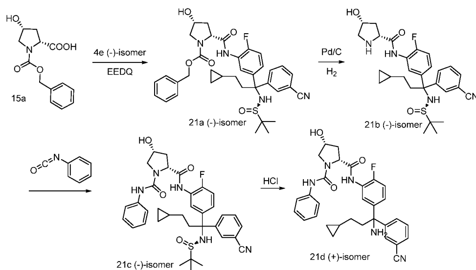
Scheme 21
