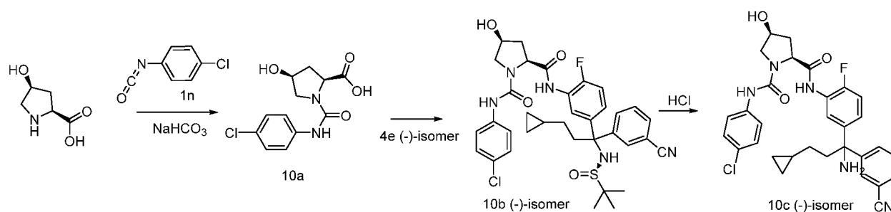
Scheme 10
