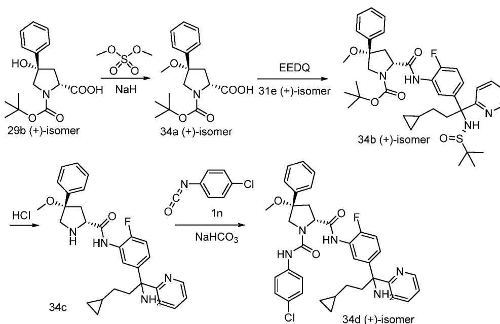
Scheme 34
