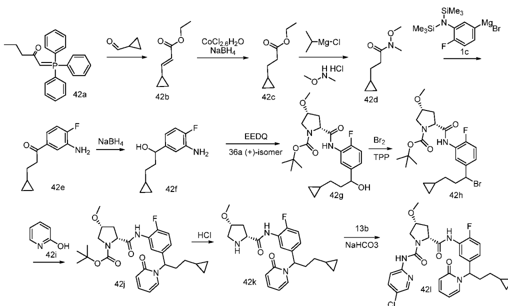
Scheme 42
