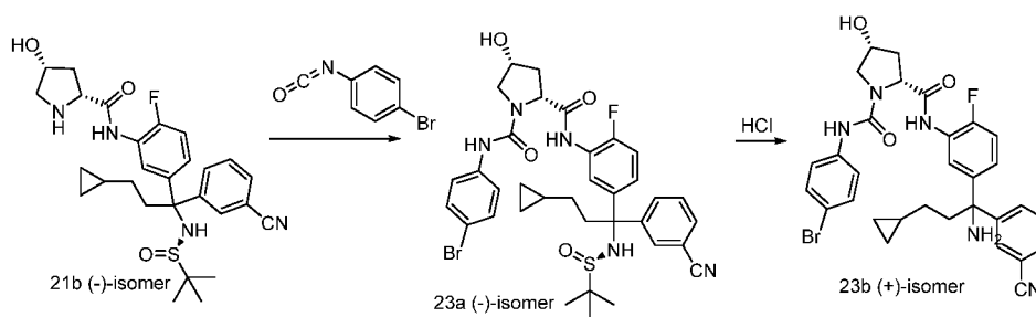
Scheme 23
