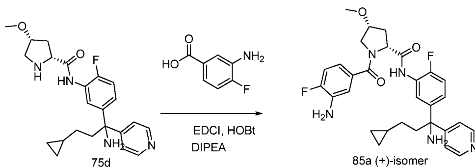
Scheme 85
