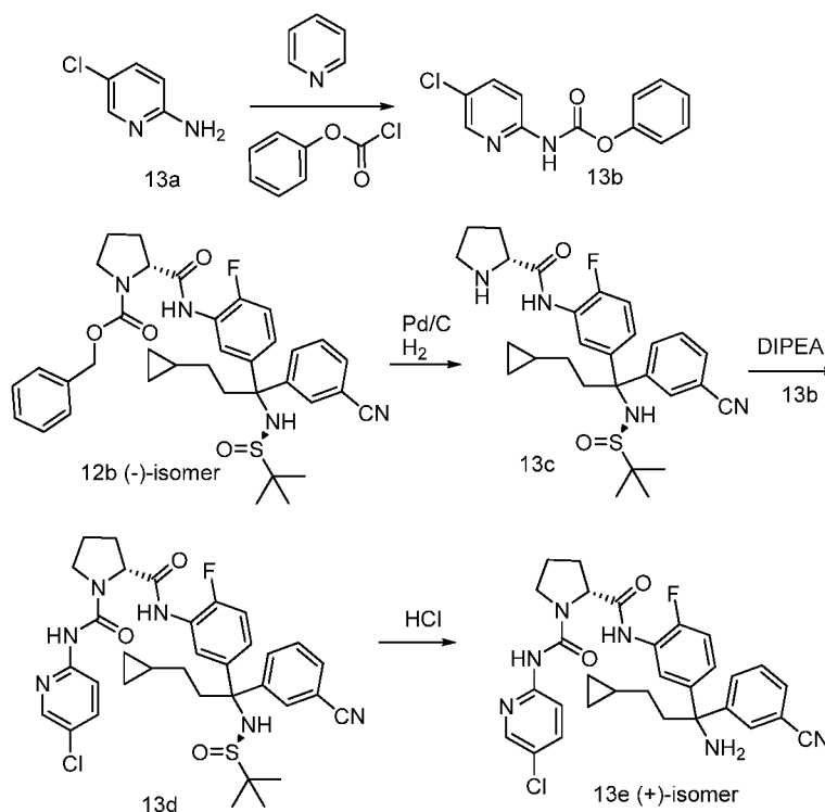
Scheme 13
