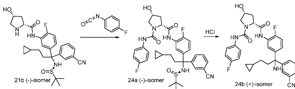
Scheme 24
