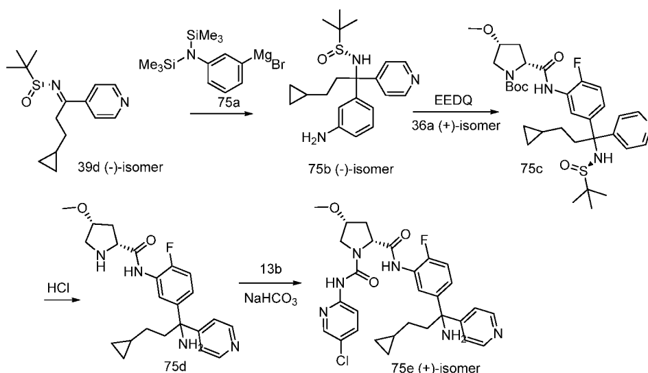
Scheme 75
