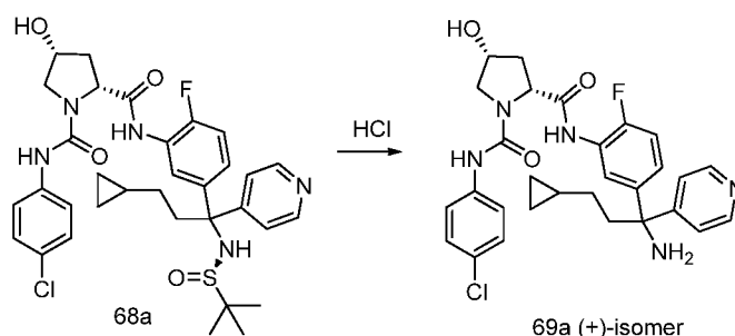
Scheme 69
