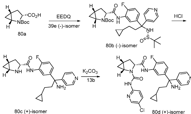
Scheme 80
