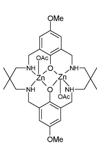
[L^3Zn_2(OAc)_2]
