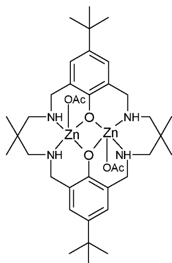
[L^1Zn_2(OAc)_2]
