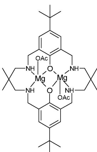
[L^1Mg_2(OAc)_2]
