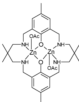
[L^2Zn_2(OAc)_2]
