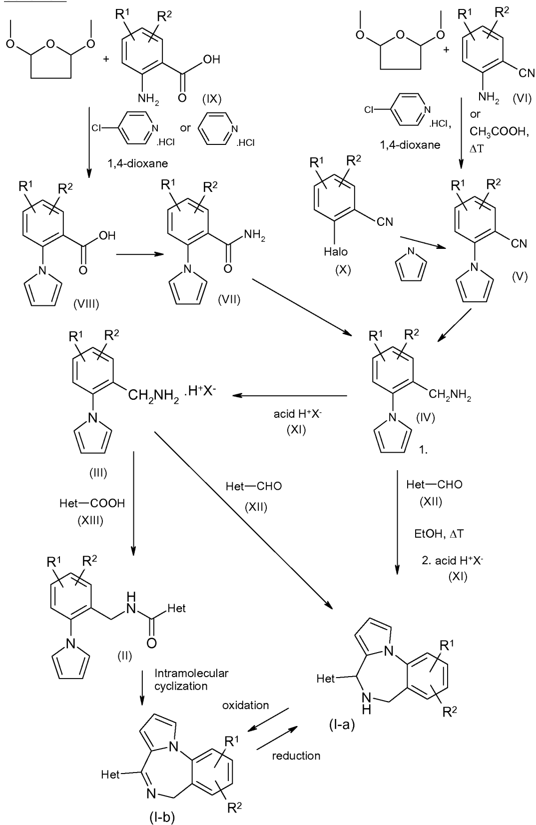
Scheme 1
