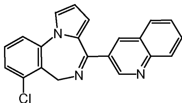
Compound 201
