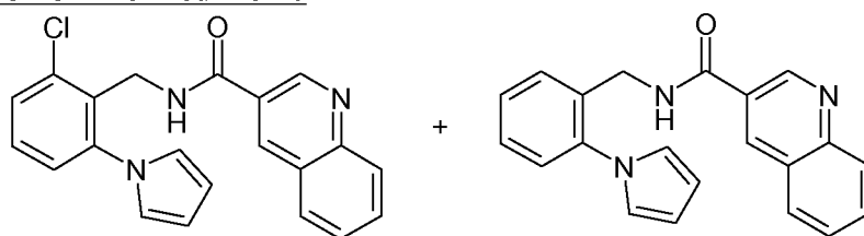
intermediate 10 (mixture)
