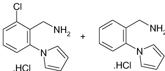
intermediate 9 (mixture)
