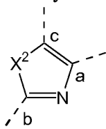
(d-2)
