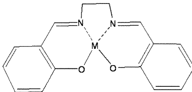
N,N'-Bis(salicylidene)ethylenediamine metal
