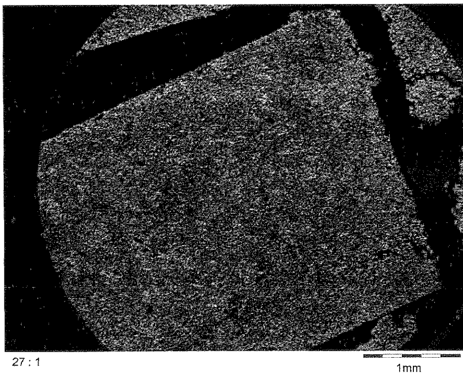
Fig. 8 c) EDX mapping of W
