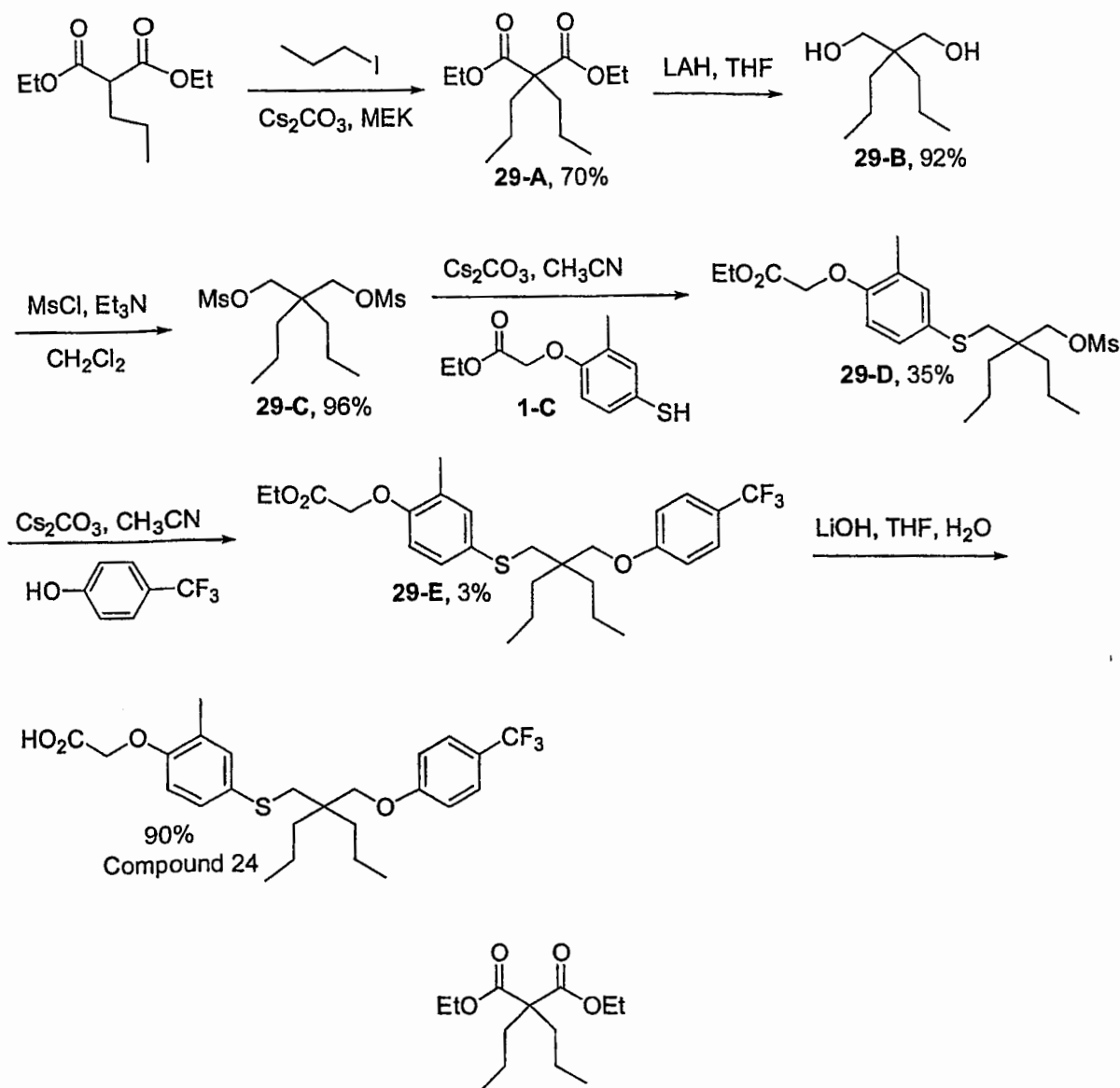
29-A 2,2-Dipropyl-malonic acid diethyl ester
