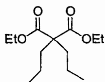
29-A 2,2-Dipropyl-malonic acid diethyl ester
