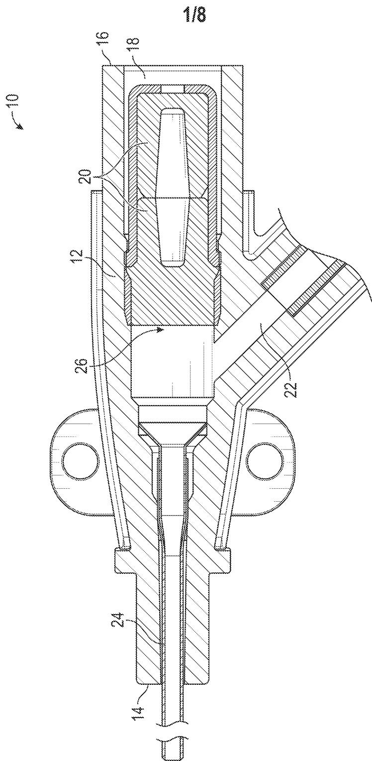
FIG. 1 (Prior Art)
