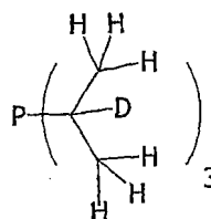
P(d_1-C_3H_7)_3
