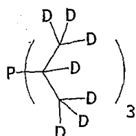
P(d_7-C_3H_7)_3
