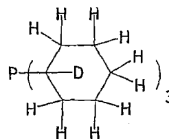
P(d_1-C_6H_{11})_3
