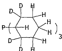
P(d_4-C_6H_{11})_3
