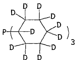
P(d_{11}-C_6H_{11})_3
