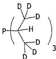
P(d_6-C_3H_7)_3
