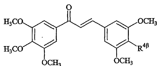
Example Table 26. 3-[4-(Heteroaryl or Heterocyclic)-3,5-dimethoxyphenyl]-1-[(3,4,5-trimethoxy)phenyl]-2-propen-1-ones.
