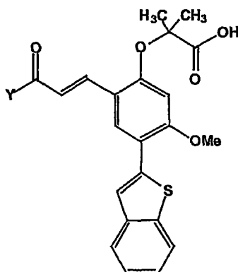
Example Table 29. Substituted 3-[5-(benzo[b]thien-2-yl)-2-(2-carboxy-2-propoxy)-4-methoxyphenyl]-1-phenyl-2-propen-1-ones.
