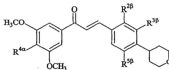
Example Table 28. Substituted 3-[4-(pyran-4-yl)phenyl]-1-[(3,5-dimethoxy)phenyl]-2-propen-1-ones.
