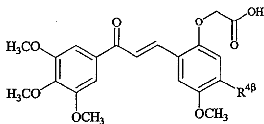
Example Table 24. 3-[4-(Heteroaryl or Heterocyclic)-2-carboxymethoxy-4-methoxyphenyl]-1-[(3,4,5-trimethoxy)phenyl]-2-propen-1-ones.
