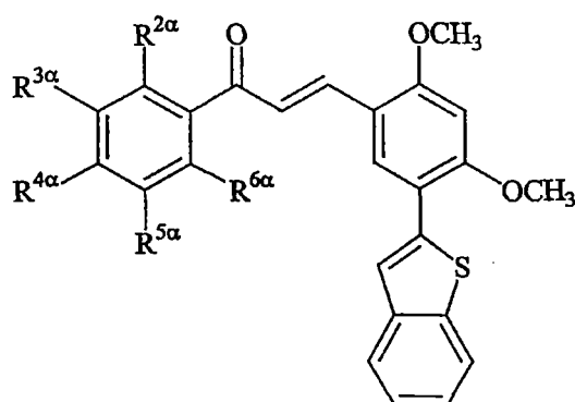
Example Table 4. Substituted 3-[5-(benzo[b]thien-2-yl)-2,4-dimethoxyphenyl]-1-phenyl-2-propen-1-ones.
