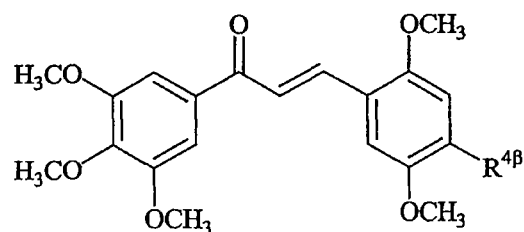
Example Table 25. 3-[4-(Heteroaryl or Heterocyclic)-2,4-dimethoxyphenyl]-1-[(3,4,5-trimethoxy)phenyl]-2-propen-1-ones.
