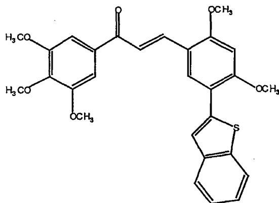
3-[5-(benzo[b]thien-2-yl)-2,4-dimethoxyphenyl]-1-(3,4,5-trimethoxyphenyl)- 2-propen-1-one
