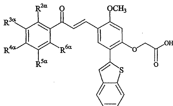
Example Table 21. Substituted 3-[5-(benzo[b]thien-2-yl)-4-carboxymethoxy-2-methoxyphenyl]-1-phenyl-2-propen-1-ones.
