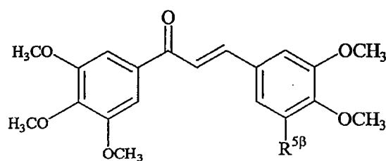
Example Table 9. 3-[5-(Heteroaryl or Heterocyclic)-3,4-dimethoxyphenyl]-1-[(3,4,5-trimethoxy)phenyl]-2-propen-1-ones.
