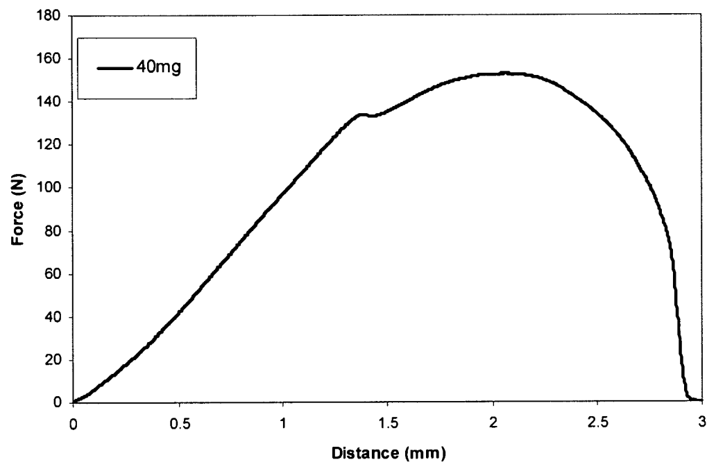
Example 20 Indentation Test of Example 14.5 tablet
