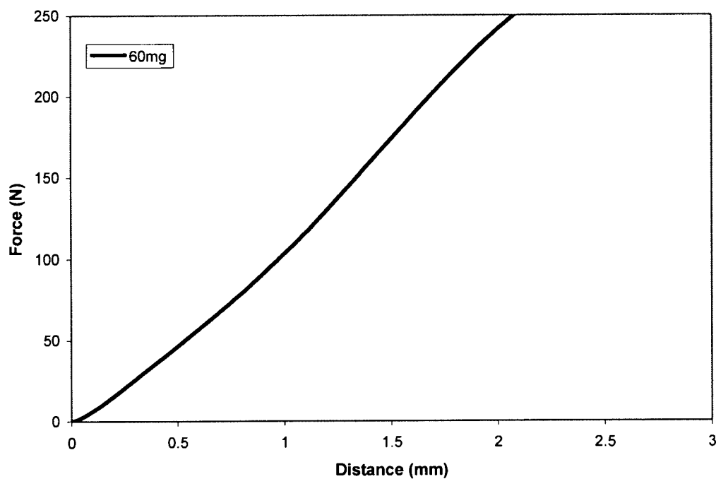
Example 20 Indentation Test of Example 17.1 tablet
