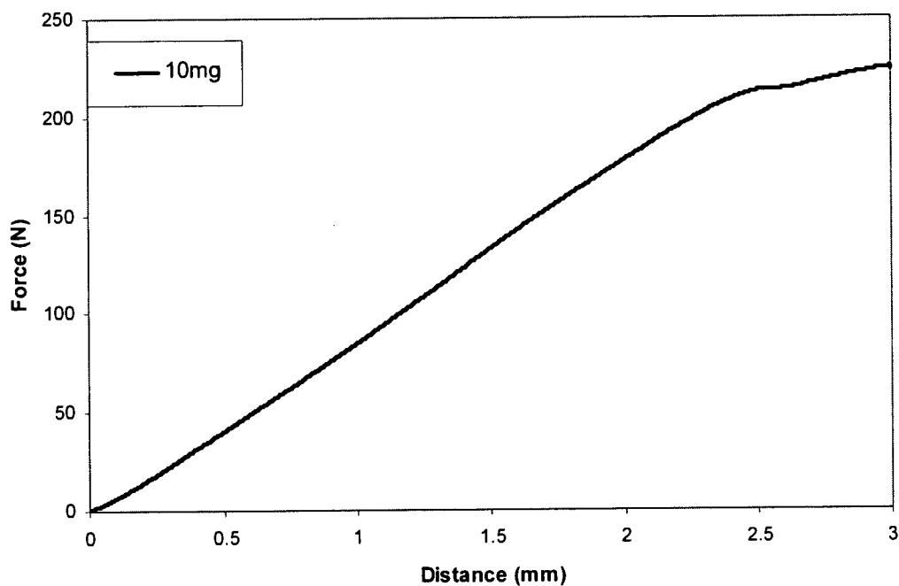
Example 20 Indentation Test of Example 14.1 tablet
