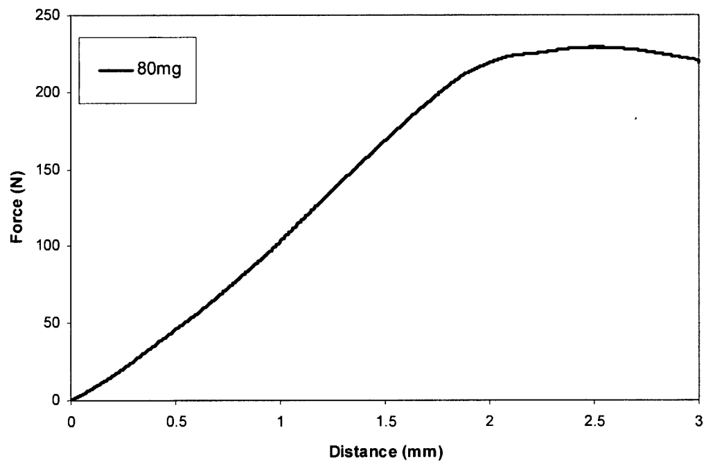
Example 20 Indentation Test of Example 16.2 tablet
