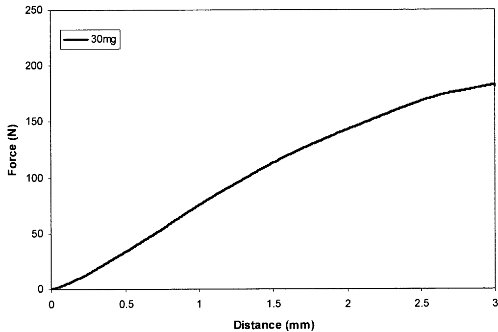
Example 20 Indentation Test of Example 13.4 tablet
