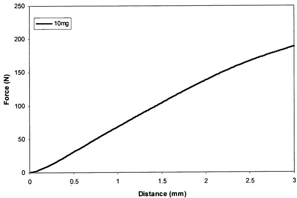
Example 20 Indentation Test of Example 13.1 tablet
