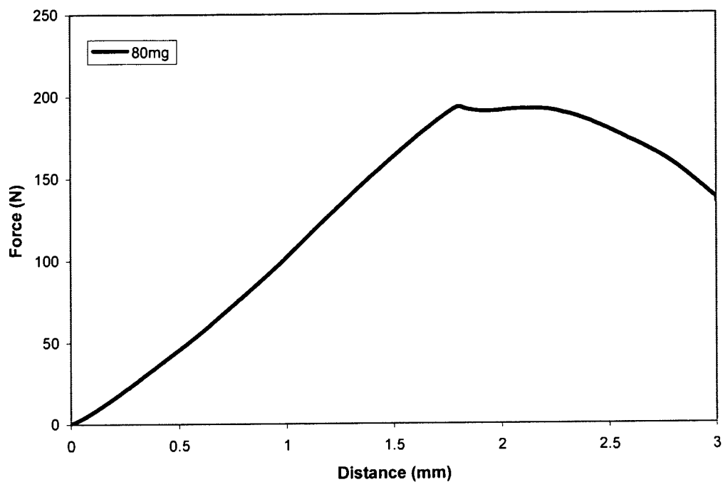
Example 20 Indentation Test of Example 18.2 tablet
