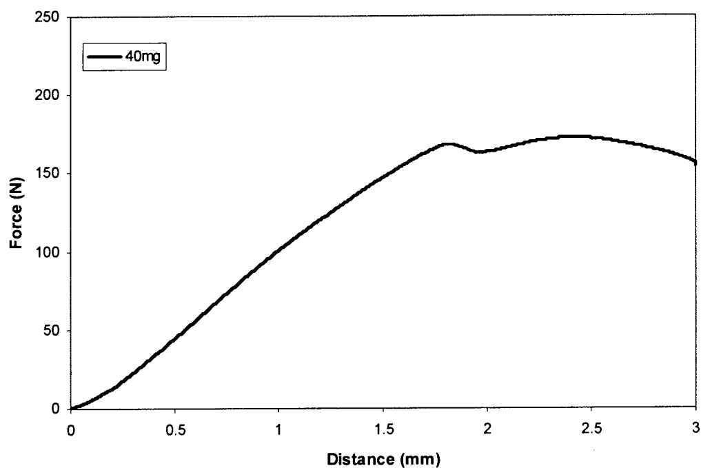
Example 20 Indentation Test of Example 13.5 tablet
