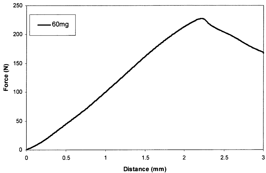
Example 20 Indentation Test of Example 16.1 tablet
