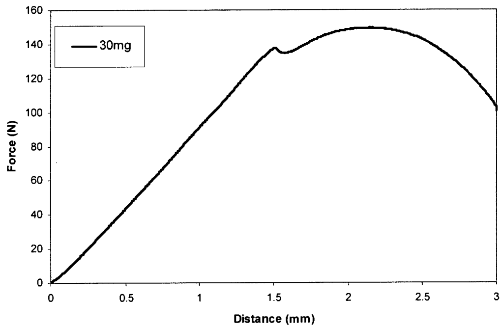
Example 20 Indentation Test of Example 14.4 tablet
