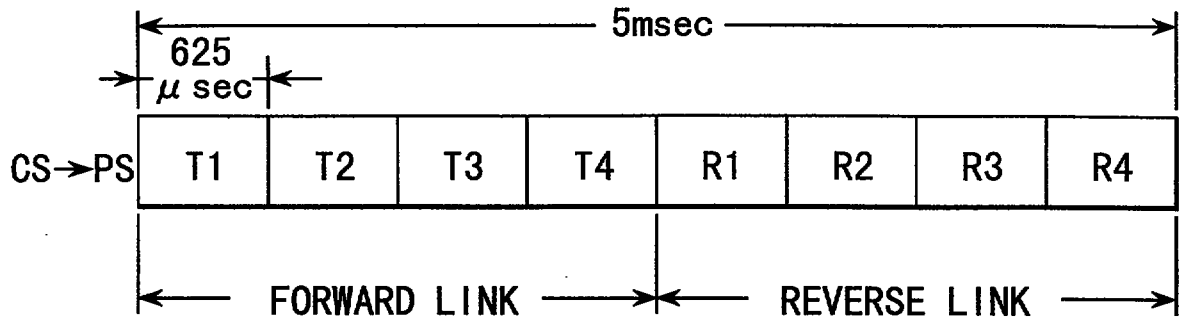
FIG. 2 (PRIOR ART)
