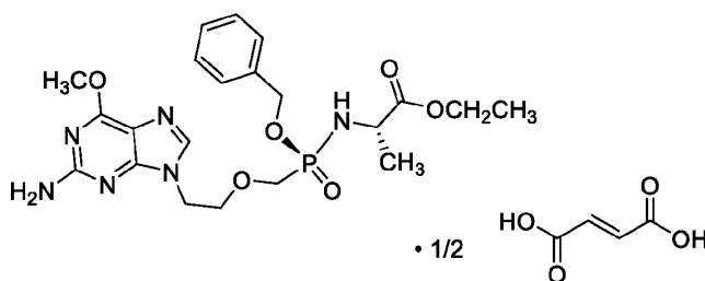
Compound V
