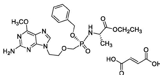
Compound II
