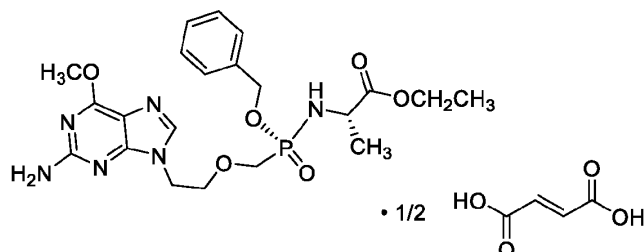
Compound IV
