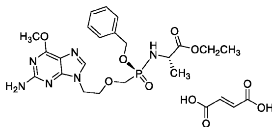
Compound III
