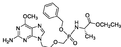
Compound I
