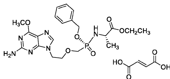
Compound II
