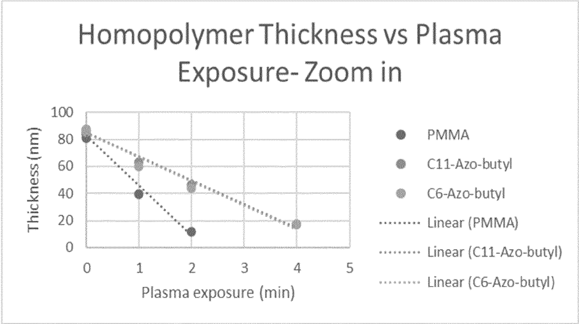
Figure 5 Homopolymer etch rate
