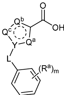
(Formula IV)
