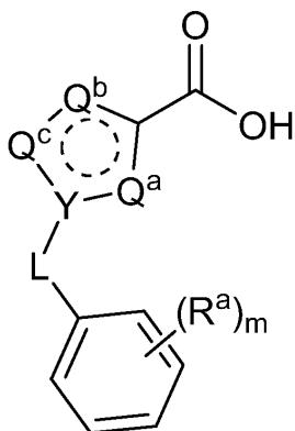
Formula IV
