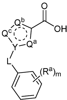
(Formula IV)
