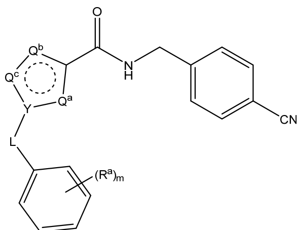
(Formula III),
