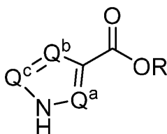
(Formula V)
