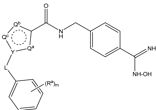
(Formula II)
