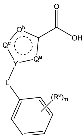
(Formula IV).
