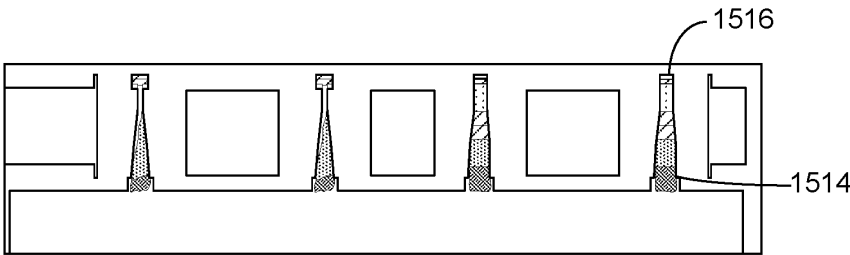
Fluid velocity contour (front view)
