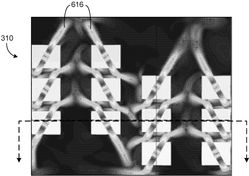
Fluid velocity contour (top view)
