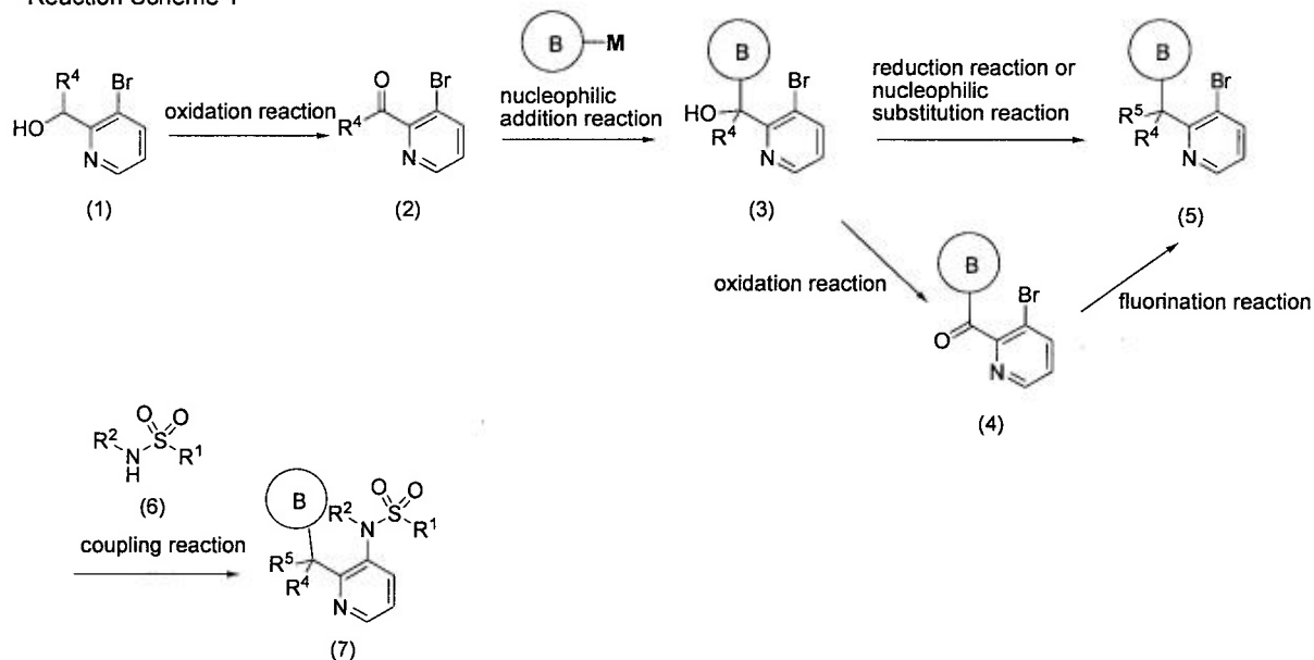
Reaction Scheme 1
