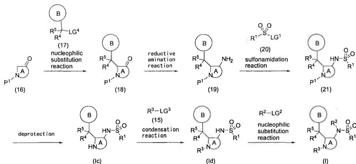
Reaction Scheme 4
