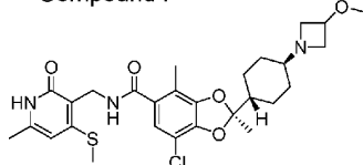
Compound I
