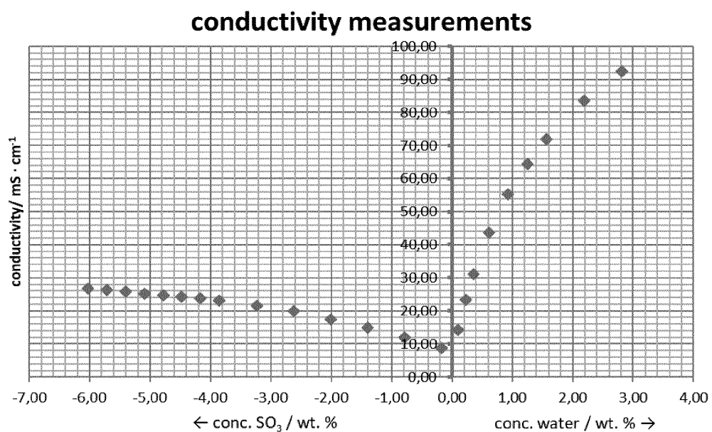
Figure 2: conductivity of water addition to a mixture of ~75,5 wt% MSA ~15 wt% H 2 SO 4 and 5 ~9,5% SO 3
