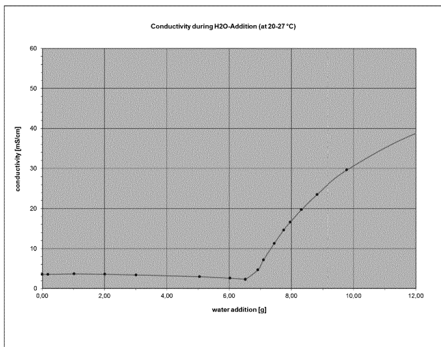
Figure 2: conductivity of water addition to a mixture of ~75,5 wt% MSA ~15 wt% H 2 SO 4 and 5 ~9,5% SO 3
