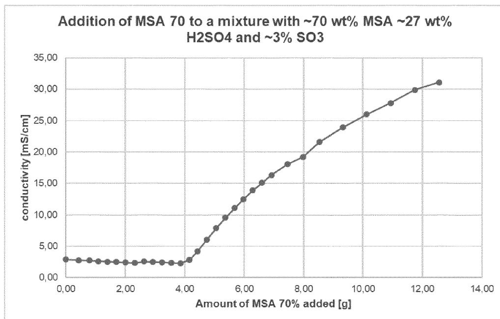
Figure 4: conductivity of MSA 70% addition to a mixture of ~70 wt% MSA ~27 wt% H 2 SO 4 and ~3% SO 3 .
