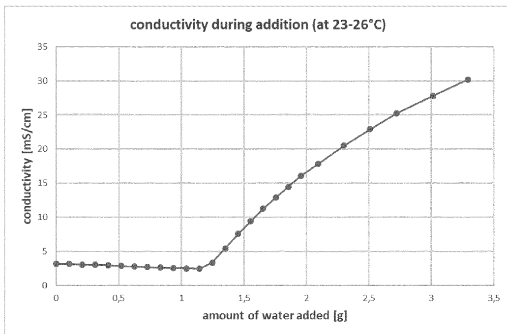
Figure 3: conductivity of water addition to a mixture of ~70 wt% MSA ~27 wt% H 2 SO 4 and ~3% SO 3
