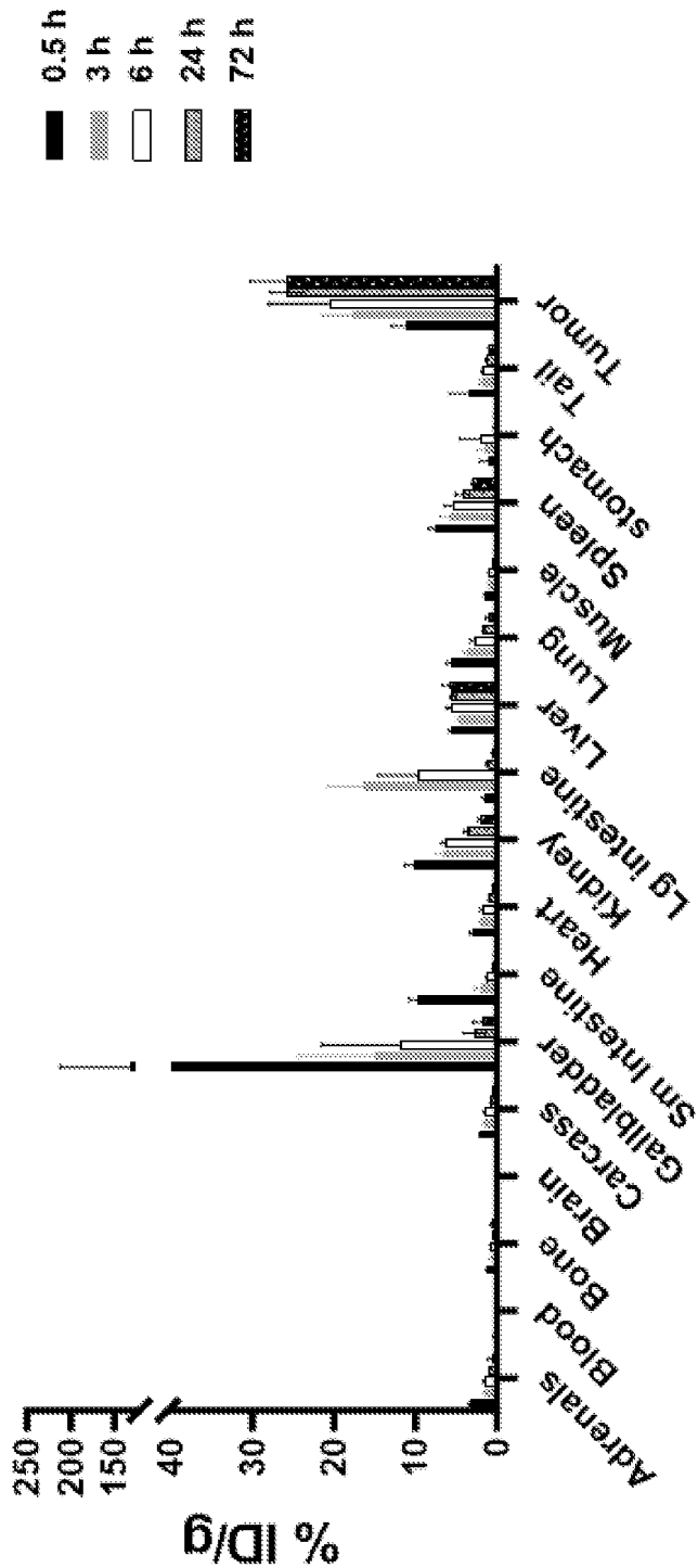
Biodistribution of ^{111}\text{In} [In]-Compound 140B in Tumor Bearing Mice
