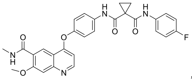
Compound 1
