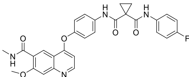
Compound 1
