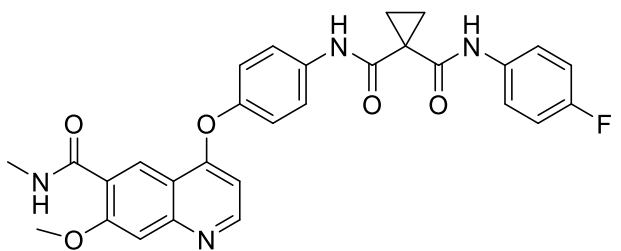
Compound 1
