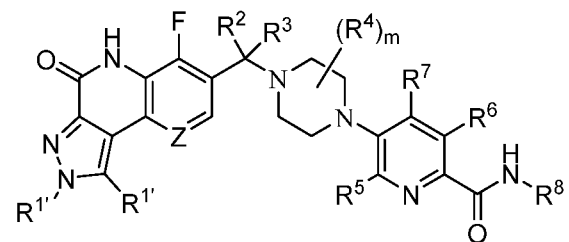
Formula (Ii);
