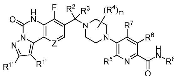
Formula (Ih);
