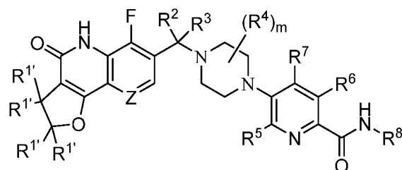
Formula (Ip);
