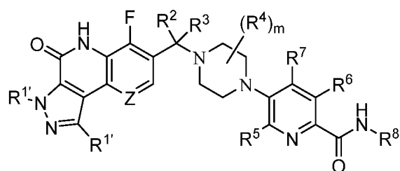
Formula (Ij);
