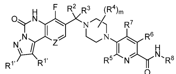
Formula (Ih);
