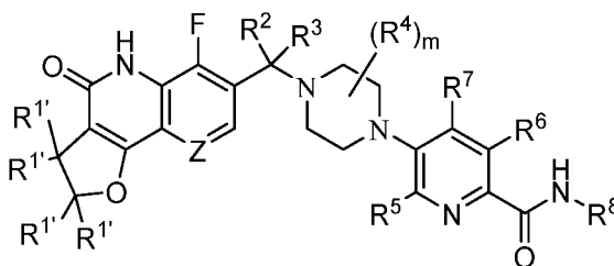
Formula (Ip);
