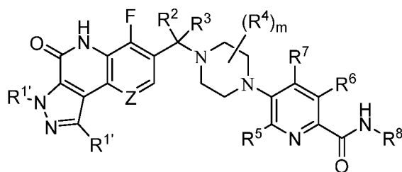
Formula (Ij);
