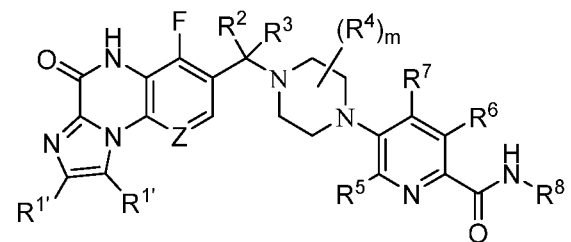
Formula (Id);
