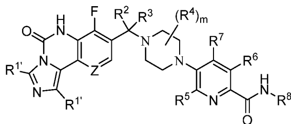
Formula (Ig);
