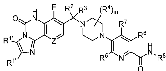
Formula (If);
