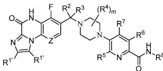
Formula (Id);
