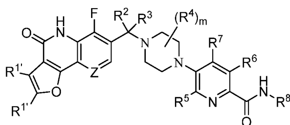
Formula (In);
