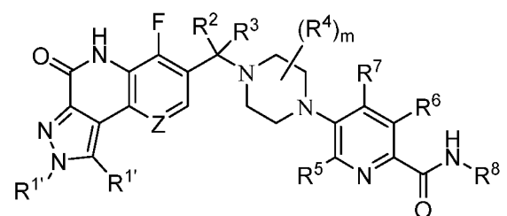
Formula (Ii);
