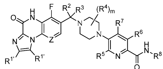
Formula (Id);
