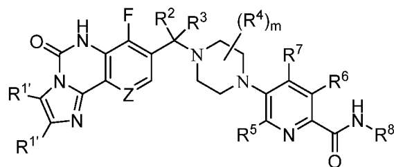
Formula (If);
