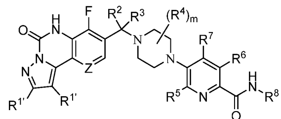
Formula (Ih);
