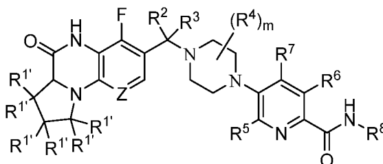
Formula (Iq);
