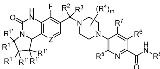
Formula (Ir);
