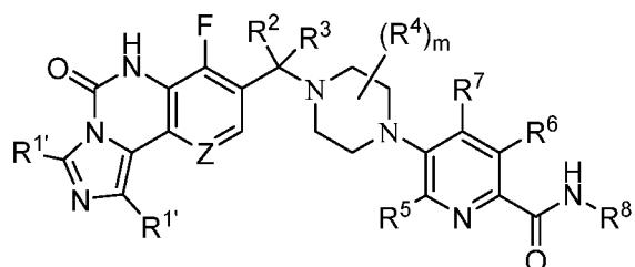
Formula (Ig);
