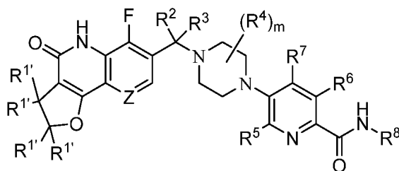
Formula (Ip);
