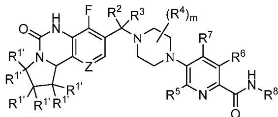
Formula (Ir);
